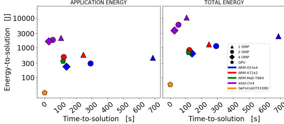
Fig. 7: Energy-to-solution (in Joule) as a function of time-to-solution (in second) for best configuration i.e. DP for CPUs and EX for GPUs. On the left panel we plot the energy-to-solution for the running kernel excluding the energy baseline, on the right panel we plot the total electric power drawn by the system running the kernel. Symbols and lines are the same as described in Figure 6.
