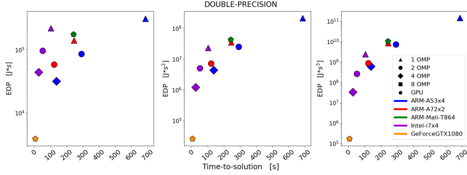
Fig. 8: EDP as a function of time-to-solution (in second) for double-precision arithmetic varying the weight of the execution time ( w = 1, 2, 3 ). Symbols and lines are the same as described in Figure 6.
