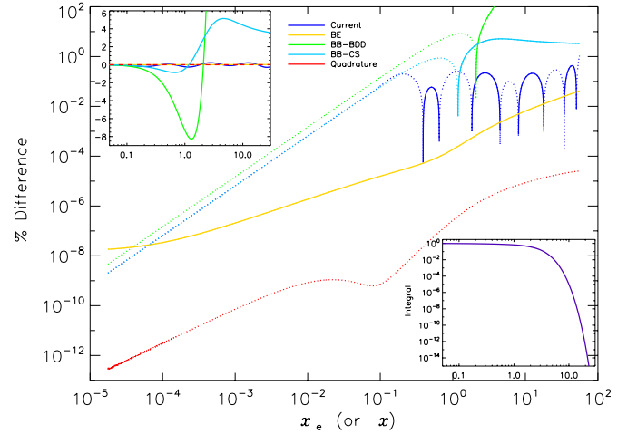
Fig. B.1. Comparison between the results of various approximations and accurate numerical integrations of Eq. (B.1). The bottom-right inset gives the numerical result derived with the NAG routine DOIAJF with a relative accuracy of 10^{-12} in the case of the blackbody spectrum. The main plot reports the per cent difference of various estimations of Eq. (B.1) with respect to the NAG DOIAJF result for the blackbody spectrum: the approximation presented here (Current, see Eq. (B.5)); the NAG DOIAJF result but for a pure BE spectrum with \mu_0 = 1.4 \times 10^{-5} (BE); the approximations reported in Burigana et al. (1991a) (BB-BDD, see Eq. (B.3)) and in Chluba & Sunyaev (2012) (BB-CS, see Eq. (B.4)); the numerical result derived with a Gaussian quadrature scheme (Press 1992) with the accuracy parameter ( EPS ) set to 10^{-9} and 2048 points in the case of the blackbody spectrum. Solid lines (or dots) correspond to positive (or negative) values. The top-left inset displays the same results of the main plot, but in a restricted frequency range and with a linear scale on the y-axis. See also the legend and the text.
