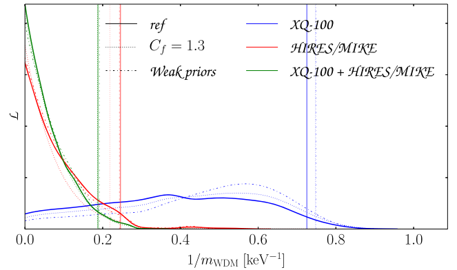
FIG. 2. One dimensional posterior likelihood distributions for the WDM mass for XQ-100, HIRES/MIKE and the combined data (blue, red and green solid curves). We also show how the results change by using a larger value for the correction factor of the XQ-100 covariance matrix (dotted curves) and using weak priors (see text) on the thermal history and cosmological parameters (dot-dashed curves). Vertical lines show the corresponding 2\sigma confidence limits.
