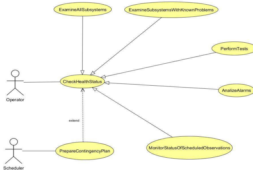
Figure 4 : CheckHealthStatus Essential Use Case
