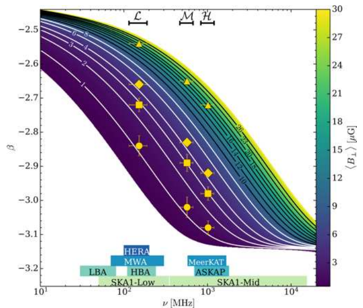
Fig. 9. A look-up plot to estimate the average value of B_\perp along a LOS, \langle B_\perp \rangle , for a given frequency \nu and brightness temperature spectral index \beta assuming the CRe spectrum by Orlando (2018). Black and white isocontours show specific values of \langle B_\perp \rangle with labels in \mu G. Yellow symbols indicate estimates of \langle B_\perp \rangle obtained from the values of \tilde{\beta} in the frequency ranges 115–189 MHz, 467–672 MHz, and 833–1200 MHz (labelled as \mathcal{L} , \mathcal{M} , and \mathcal{H} , respectively), at a common resolution of 6.7' , for the different POS of the two simulation snapshots (circles: POS yz in the strong field case; squares: POS yz in the weak field case; diamonds: POS xy and zx in the weak field case; triangles: POS xy and zx in the strong field case). Rectangles at the bottom of the plot show the frequency ranges of the low and high band antenna of LOFAR (LBA and HBA, respectively), the low and mid frequency bands of SKA (SKA1-Low and SKA1-Mid, respectively), and SKA pathfinders and precursors: the Hydrogen Epoch or Reionisation (HERA); the Murchison Widefield Array (MWA); the Karoo Array Telescope (MeerKAT); the Australian SKA Pathfinder (ASKAP).
