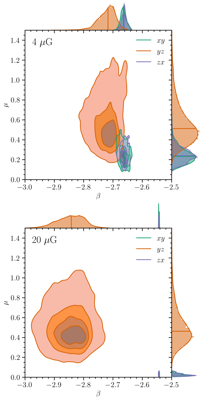
Fig. 6. Bivariate distribution of the ratio between the standard deviation of B_{\perp} and its median value, \mu , and the brightness temperature spectral index, \beta , computed in the frequency range 115–189 MHz for each LOS for the weak and strong field case (upper and lower panel, respectively), at a resolution of 6.7' . The POS are identified by the three different colours displayed in the legend. Isodensity contours are plotted at 5%, 30%, 50%, and 75% levels. The histograms above and to the right of the main plots show the marginal distribution of the two quantities. The median values are marked by horizontal and vertical lines and listed in Table 3.
