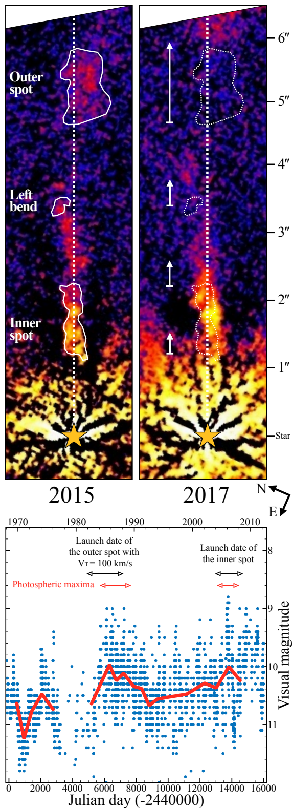
Fig. 3. Jet of RY Tau from the H3 images tracing the [\text{Fe II}] emission at 1.64 \mu\text{m} from the jet. Top panel: comparison of the jet radial extent between 2015 and 2017. The 2015 features identified in both images are replicated as dash contours in the 2017 image. The arrows represent their apparent motion. The jet axis (P.A.= 293^\circ ) is indicated by the dashed line. The bright signal in the inner 1'' is primarily stellar flux residual. Bottom panel: the stellar lightcurve in the last 50 years. The red lines is the best fit to the 3100 blue datapoints. The calculated launch date of the inner and outer jet spots are indicated by the black arrows, while the red arrows highlight the local photospheric maxima from the curve.
