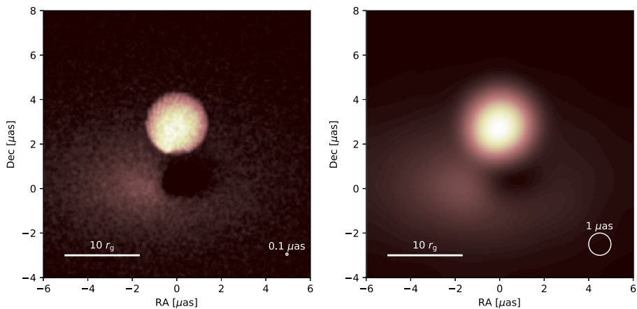
Fig. 3 Image of an example geometry of an AGN core: a spatially extended hot corona is located above an accretion disc that surrounds the central black hole, assuming the same system parameters as in Fig. 2. The corona is the primary source of X-ray photons that reflect from the accretion disc. Left: Image blurred by 0.1 \mu\text{as} FWHM 2D Gaussian (indicated by the white circle). Right: The same model blurred by a 1 \mu\text{as} Gaussian. Image brightness is linearly proportional to the photon count
