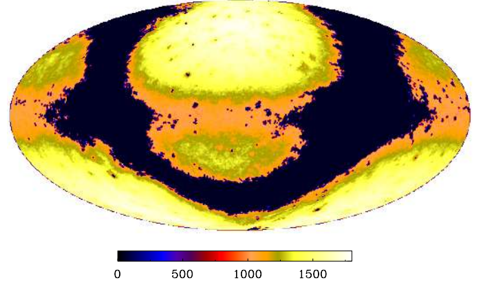
Fig. 25. Expected counts of GC galaxies (with reliable spectroscopic redshifts) in deg ^{-2} (see text) in ecliptic coordinates. Here the number counts decrease faster with latitude than for the WL counts (cf. Fig. 24) since the impact of stars (spectra) from our Galaxy on the GC one-dimensional spectra is more severe than the impact of stars (point-like) on the two-dimensional WL data.
