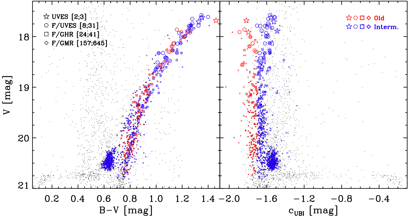
Fig. 1. Left: brighter portion of the CMD of the Carina dwarf in the V vs. B-V plane. The large colored circles represent the spectroscopic targets in this investigation. The color coding derives from the selection criteria shown in the right panel . Right: V vs. c_{U,B,I} diagram for the same stars. This particular color combination, (U-B)-(B-I) , allows us to split the RGB into old and intermediate-age populations (Monelli et al. 2014).
