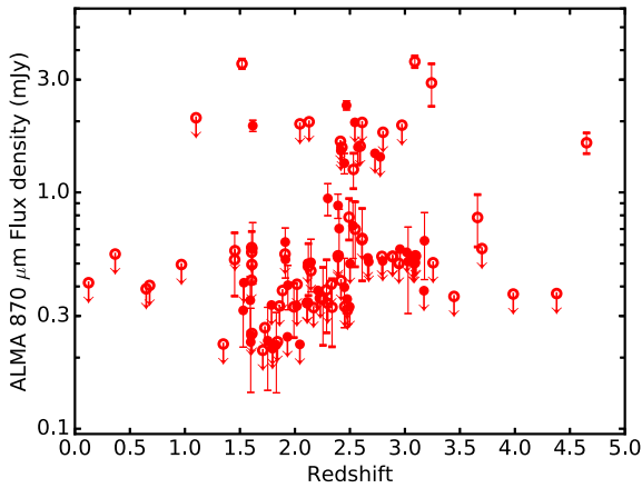
Figure A2. ALMA 870 \mu\text{m} flux density versus redshift for the X-ray detected that lie within our ALMA observations. The error bars represent the 1\sigma error on the flux density.
