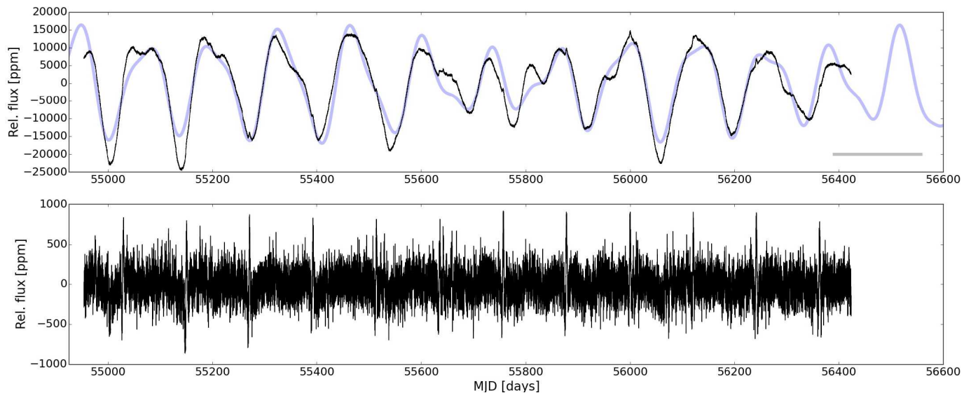
Fig. 1. Light curve of KIC9163796. The top and lower panels show the full light curve ( Q_0 – Q_{17} ), smoothed with a filter of 150 and 4 days, respectively. The synthetic light curve, depicted as solid light grey line is calculated from the four significant frequencies from Table 2. The time base of the spectroscopic monitoring is indicated through the horizontal grey bar.
