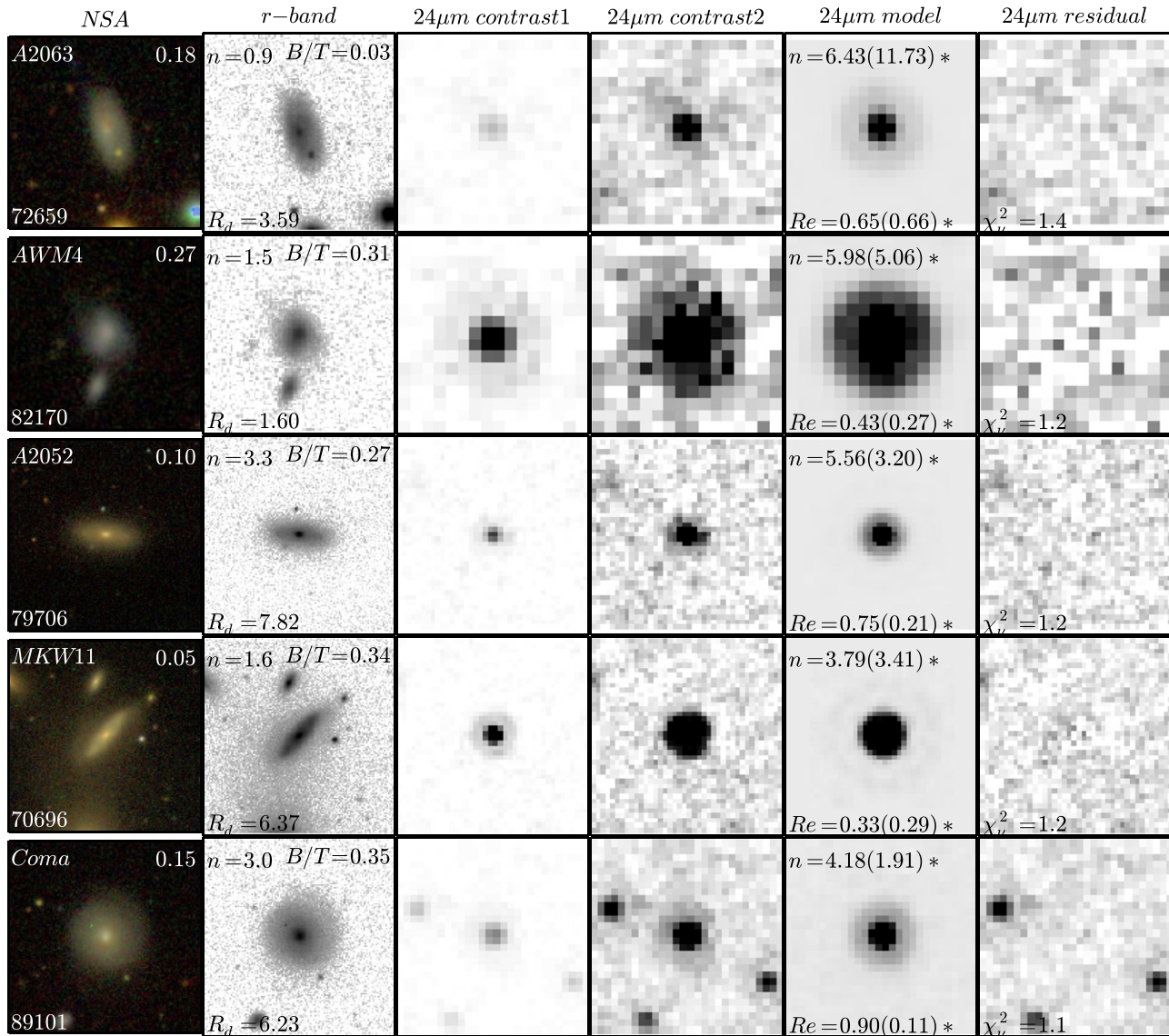
Figure 7. Example GALFIT modeling results for five randomly selected galaxies with R_{24}/R_d between 0 and 0.3. Columns 1 and 2 show the SDSS color and r -band images. Columns 3 and 4 show the 24\mu\text{m} image at two different stretches to emphasize the high and low surface-brightness features, respectively. Columns 5 and 6 show the 24\mu\text{m} single-component Sérsic model and residual, and the contrast is identical to column 4 to emphasize the low surface-brightness features. The text in column 1 gives the parent cluster, the NSA ID, and R_{24}/R_d . Column 2 lists the r -band Sérsic index n , the bulge-to-total ratio, and the disk scale length in arcseconds. The text in column 5 lists the 24\mu\text{m} Sérsic index and effective radius in arcseconds, and column 6 lists \chi^2_\nu of the best-fit model.
