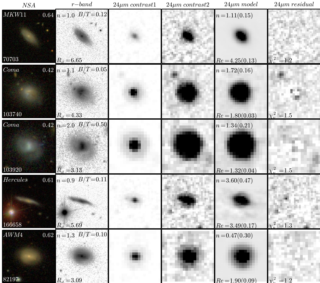
Figure 8. Example GALFIT modeling results for five randomly selected galaxies with R_{24}/R_d between 0.4 and 0.7. Columns 1 and 2 show the SDSS color and r -band images. Columns 3 and 4 show the 24\mu\text{m} image at two different stretches to emphasize the high and low surface-brightness features, respectively. Columns 5 and 6 show the 24\mu\text{m} single-component Sérsic model and residual, and the contrast is identical to column 4 to emphasize the low surface-brightness features. The text in column 1 gives the parent cluster, the NSA ID, and R_{24}/R_d . Column 2 lists the r -band Sérsic index n , the bulge-to-total ratio, and the disk scale length in arcseconds. The text in column 5 lists the 24\mu\text{m} Sérsic index and effective radius in arcseconds, and column 6 lists \chi^2_{\nu} of the best-fit model.
