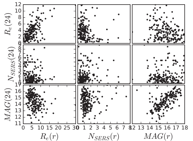
Figure 6. GALFIT 24\ \mu\text{m} model parameters versus Simard et al. (2011) r -band model parameters for all galaxies in our final sample. The top-left and bottom-right panels show that 24\ \mu\text{m} and r -band effective radius and magnitude are strongly correlated.
