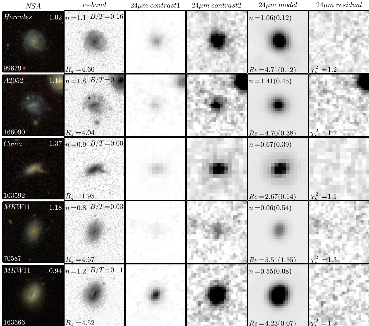
Figure 9. Example GALFIT modeling results for five randomly selected galaxies with R_{24}/R_d greater than 0.9. Columns 1 and 2 show the SDSS color and r -band images. Columns 3 and 4 show the 24\mu\text{m} image at two different stretches to emphasize the high and low surface-brightness features, respectively. Columns 5 and 6 show the 24\mu\text{m} single-component Sérsic model and residual, and the contrast is identical to column 4 to emphasize the low surface-brightness features. The text in column 1 gives the parent cluster, the NSA ID, and R_{24}/R_d . Column 2 lists the r -band Sérsic index n , the bulge-to-total ratio, and the disk scale length in arcseconds. The text in column 5 lists the 24\mu\text{m} Sérsic index and effective radius in arcseconds, and column 6 lists \chi^2_{\nu} of the best-fit model.
