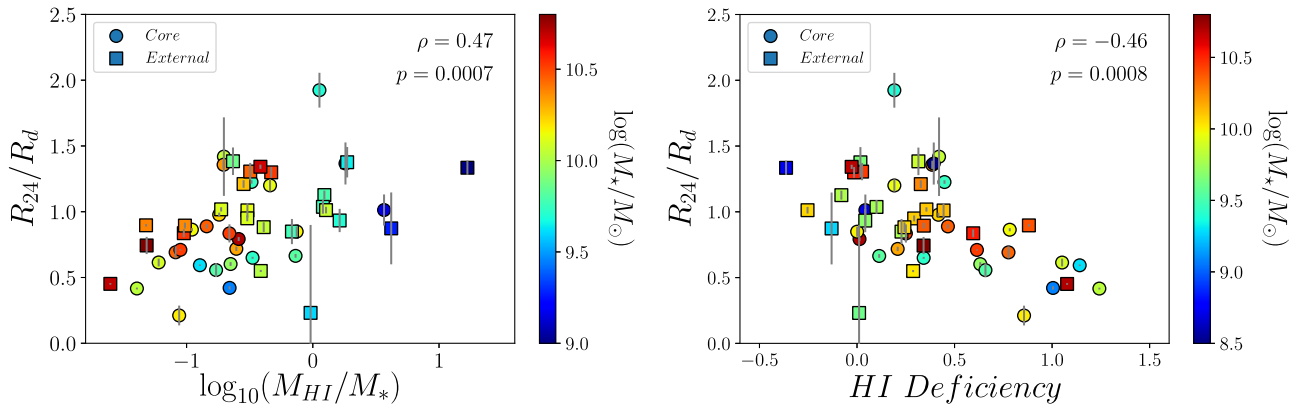
Figure 16. (Left) R_{24}/R_d versus HI mass fraction. The data show a significant ( >3\sigma ) correlation between R_{24}/R_d and HI mass fraction. (Right) R_{24}/R_d versus HI deficiency. The data show a significant ( >3\sigma ) anti-correlation between R_{24}/R_d and HI deficiency in the sense that galaxies with smaller R_{24}/R_d also have less HI gas than isolated galaxies.
