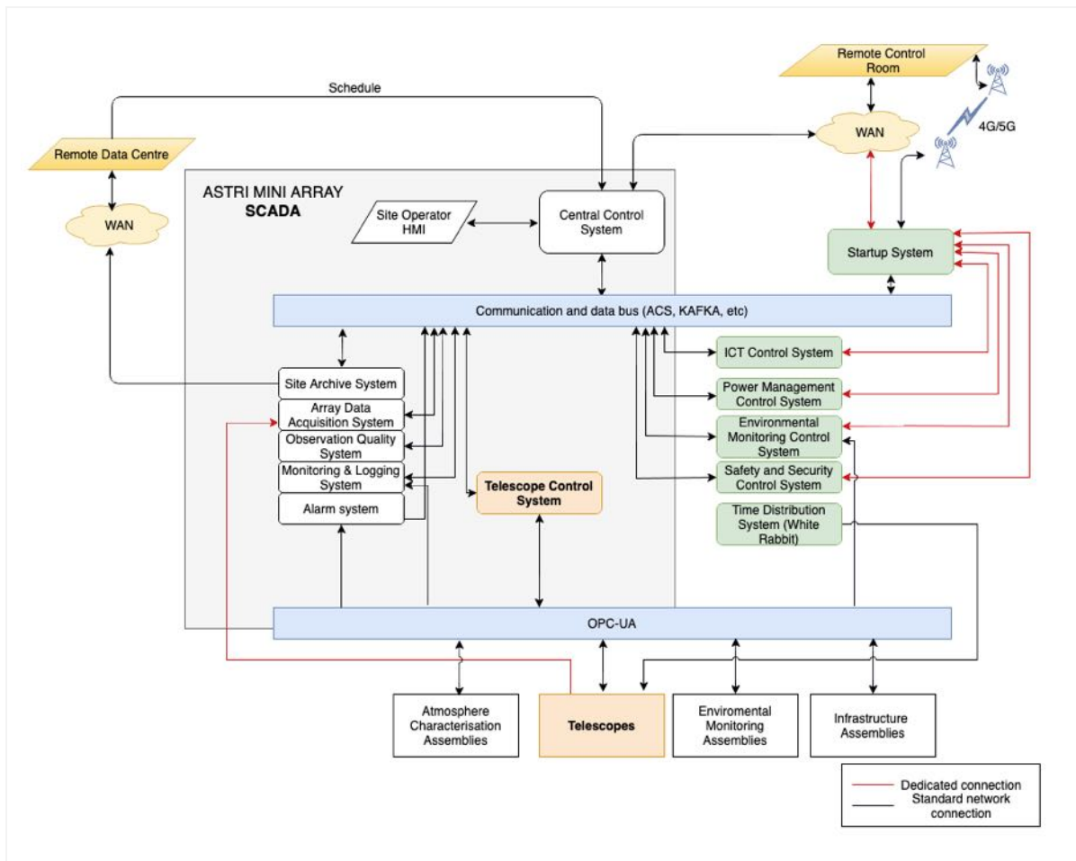
Figure 27: Data and control flow between the main subsystems of the SCADA System and the Startup System.
