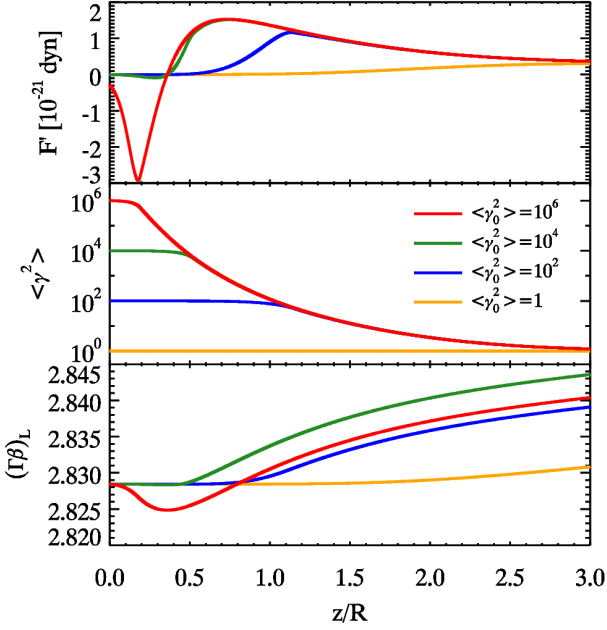
Figure 9. Radiative acceleration of the sheath due to variation of the average internal energy content of the sheath ( \langle \gamma^2 \rangle ) from 1 to 10^6 for a constant isotropic spine luminosity L_{\text{iso,S}} = 10^{45} erg s ^{-1} , a constant spine Lorentz factor \Gamma_S = 15 and for an initial sheath Lorentz factor \Gamma_L = 3 . The x-axis depicts the position z normalized by the vertical structure dimension R . Top panel depicts the radiative force measured in the layer frame. Middle panel: the internal energy of the sheath denoted by \langle \gamma^2 \rangle . Bottom panel: Lorentz factor of the sheath (\Gamma\beta)_L measured in the observer frame.
