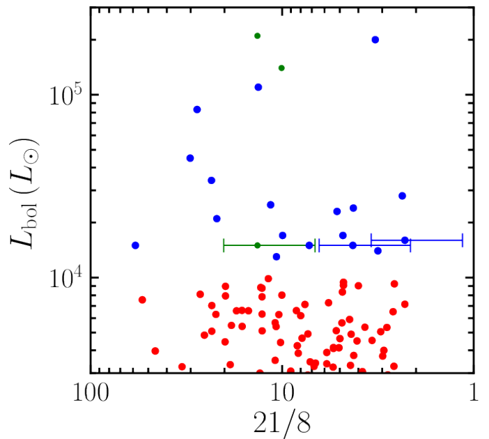
Fig. 1. Sample selection plot where the luminosity (in units of L_{\odot} ) is plotted against the MSX 21/8\mu\text{m} color. Horizontal bars mark uncertainties in the color. While the blue sources fulfill our selection criteria, the red ones are below our luminosity cut of 10^4 L_{\odot} . Green sources are those for which high-resolution mm data already exist and which were therefore excluded from the observations.
