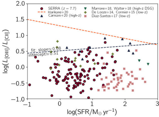
Figure 13. [O III]-to-[C II] ratio as a function of SFR. We plot the collection of observations obtained for normal high- z galaxies ( \text{SFR} < 100 M_{\odot} \text{yr}^{-1} ; Carniani et al. 2020) and dusty star-forming galaxies ( \text{SFR} > 100 M_{\odot} \text{yr}^{-1} ; Marrone et al. 2018; Walter et al. 2018), along with data for local normal (Díaz-Santos et al. 2017) and dwarf (De Looze et al. 2014; Cormier et al. 2015) galaxies. We also plot the fits from Harikane et al. (2020) and Carniani et al. (2020, computed in the present, best-fitting parameters indicated in the figure).
