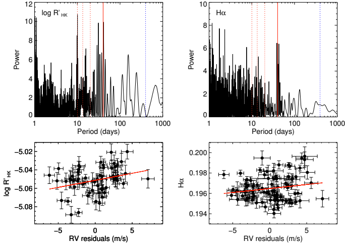
Fig. 4. Upper panels: periodograms of the \log R'_{\text{HK}} (with S/N > 20 ) and of the H \alpha indices for HARPS-N data. The red solid line indicates the 40.2 d period, the red dotted lines represent its 1st, 2nd and the 3rd harmonics; the blue dotted line indicates the period of planet b. Lower panels: correlation with the RV residuals.
