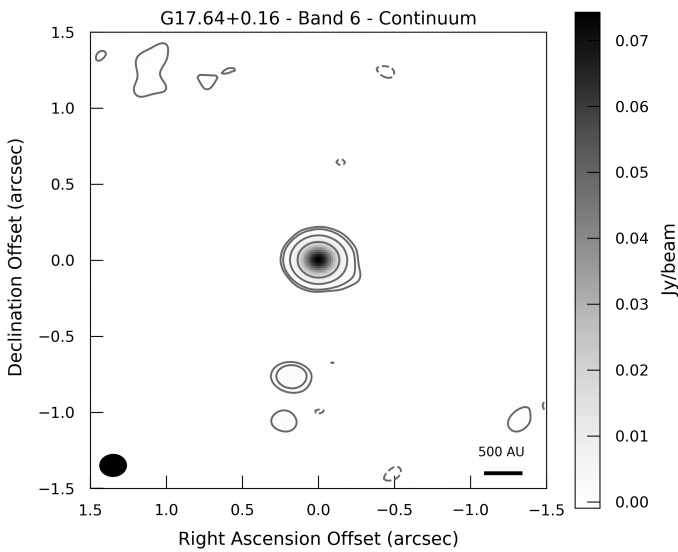
Fig. 1. ALMA band 6 (1.3 mm) continuum image of G17.64 made with a robust 0.5 value. The contour levels are set at -3, 5, 10, 50 and 200 \sigma ( 1 \sigma = 0.07 \text{ mJy beam}^{-1} ) to indicate the weak southern sources and the strength of G17.64 (negative contours are dashed lines). The map is centred (0,0) on G17.64 at J2000 18^{\text{h}}22^{\text{m}}26.385^{\text{s}} -13^{\circ}30'11.97'' . The synthesised beam is indicated to the bottom left of the figure, while a scale bar is shown in the bottom right.
