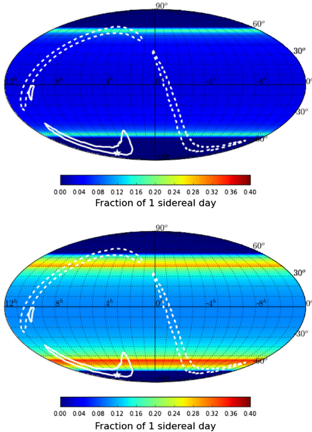
FIG. 1. Sky map in equatorial coordinates where the color scale indicates the fraction of one sidereal day for which a pointlike source at declination \delta is visible to the SD of the Auger Observatory (latitude \lambda = -35.2^\circ ) at zenith angle 90^\circ < \theta < 95^\circ (top panel), and 75^\circ < \theta < 90^\circ (bottom panel). The white solid lines indicate the 90% C.L. contour position of GW150914 [1,2] and the dashed white lines indicate the corresponding 90% C.L. contour position of GW151226 [3,4]. The white star indicates the best-fit position of the GW150914 event obtained in combination with data from the Fermi-GBM instrument (see Fig. 10 in [7]).
