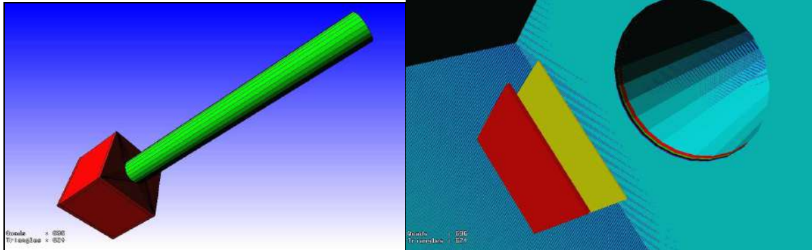
Figure 4-49: (Left panel) the simulated NHXM001 geometry; (Right panel): a detail of the detectors and collimator of the NHXM001 geometry.
