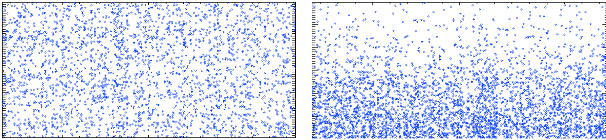
Figure 7: expanded beam uniformity (left) when the source is vertically aligned at z = 0 and (right) vertically misaligned at z = -150 \mu\text{m} . The full field is 170 \text{ mm} \times 60 \text{ mm} .
