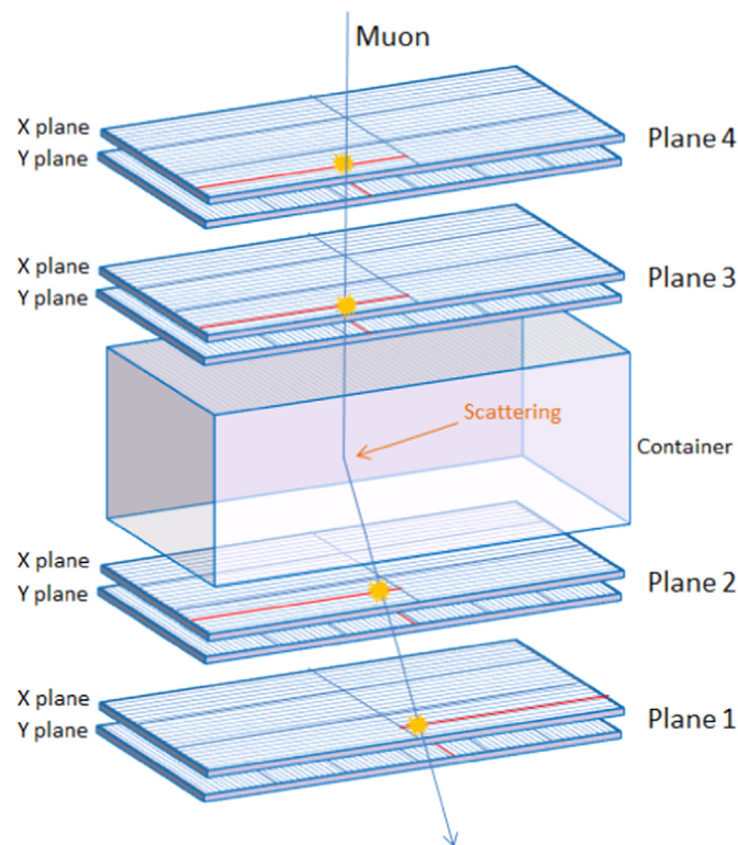
Fig. 1. Schematic representation of the Muon Portal Detector (not in scale). The eight planes provide 4 ( X,Y ) points that are used to reconstruct the track before and after passing through the container. The size of each plane is 3 \times 6 \text{ m}^2 .
