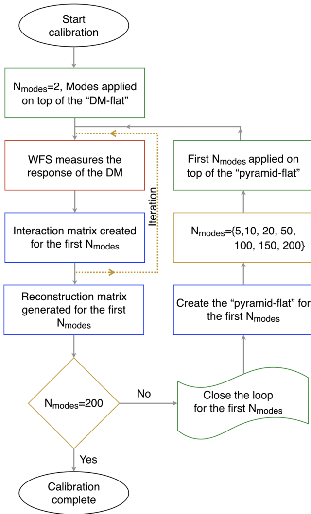
Fig. 7 Flowchart explaining the calibration procedure of the mother- \text{IMM} for 200 modes. A Python script communicates with the instrument and performs the calibration in an almost fully automatic way.
