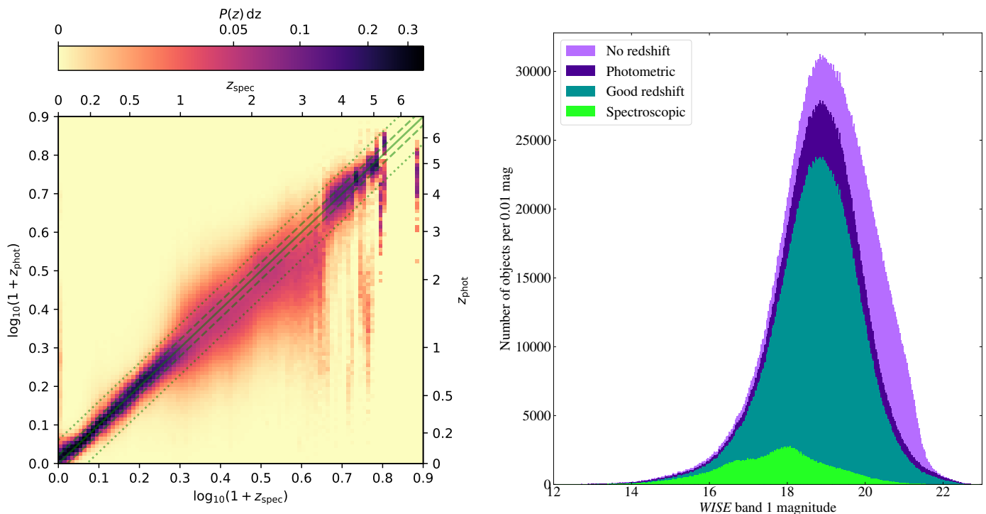
Fig. 9. Statistics of the photometric and spectroscopic redshifts. Left: Photo- z posterior distributions as a function of SDSS spectroscopic redshift (zwarning_sdss = 0) and photo- z estimates that pass the photo- z quality selection (flag_qual = 1). The photo- z distribution is normalized such that the distribution for each z_{\text{spec}} bin integrates to unity. Dashed and dotted lines illustrate the bounds z_{\text{phot}} = z_{\text{spec}} \pm 0.05 and 0.15 \times (1 + z) respectively. Right: the distribution of available redshifts for all optically identified objects as a function of WISE band 1 magnitude, where a ‘good redshift’ is defined in the text.
