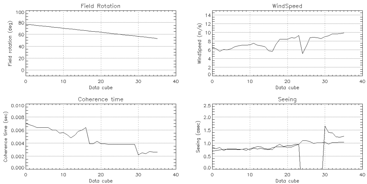
Figure 1 Observational conditions as retrieved from the fits headers. Field rotation (top left), wind speed (top right), correlation time tau0 (bottom left) and seeing (bottom right). The data cube number is indicated on the horizontal axis, i.e. each data cube is about 1 minute.
