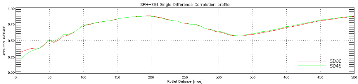
Figure 8 Single Difference: Correlation profiles. (top panel) Map of correlation coefficient of SD00 (left) and SD45 (right). (bottom panel) Azimuthal average profiles of SD00 and SD45 correlation coefficients. We observe a very close match between the two SD profiles.
