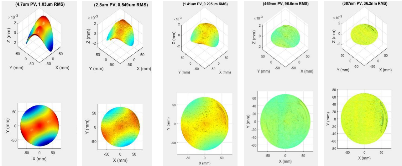
Before polishing After run #5 After run #10 After run #19 After run #21 Shape: 1030 nm rms Shape: 549 nm rms Shape: 295 nm rms Shape: 97 nm rms Shape: 36 nm rms Roughness: 6 nm rms Roughness: 21 nm rms Roughness: 29 nm rms Roughness: 18 nm rms Roughness: 9 nm rms
