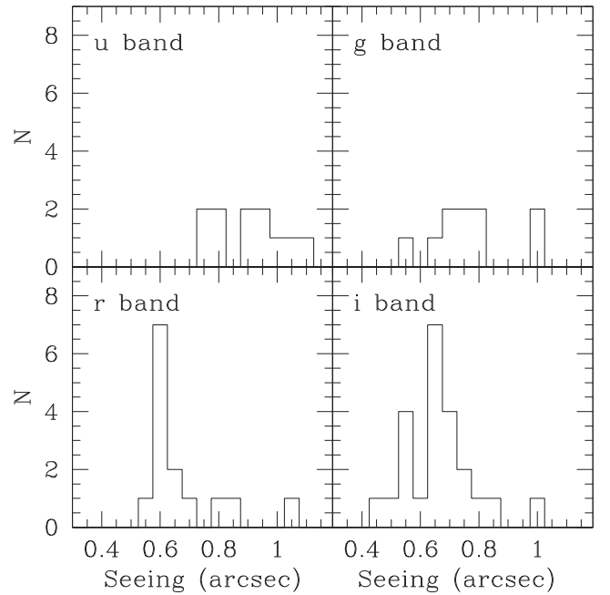
Figure 2. Seeing distribution in the four observed bands (see text).
