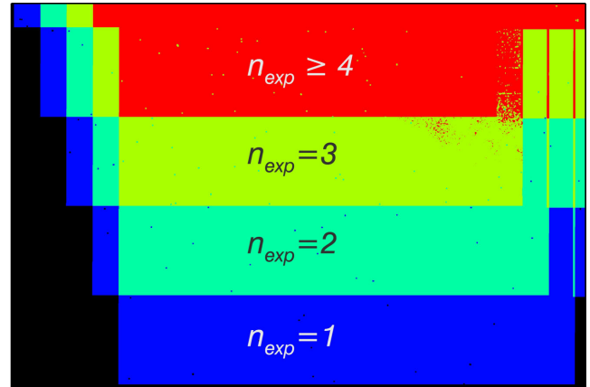
Figure 7. Cut-off of an exposure mask near to a corner of a VST image. The area shown is about 14 \times 12 arcmin ^2 . The colours correspond to the different numbers of exposure as indicated.
