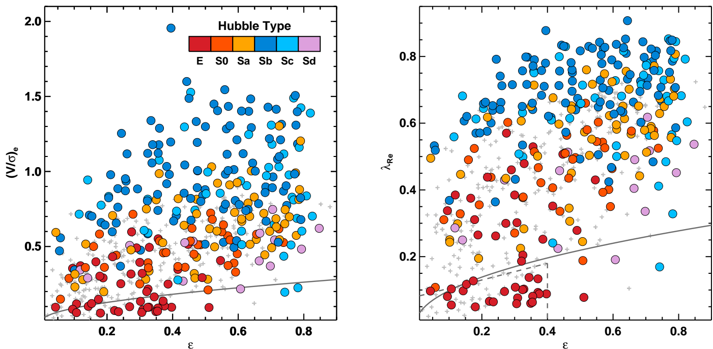
Fig. 4 (V/\sigma)_e (left) and (\lambda_{Re}, \epsilon) (right) relations for the CALIFA sample of 300 galaxies. Galaxies are color-coded with Hubble type as indicated by the colorbar. For reference, we plot the ATLAS 3D sample with gray crosses. The solid line demarcates the division between Slow and Fast rotators as established by Emsellem et al. (2011). The dashed line in the right panel marks the revised division between Slow and Fast rotators defined by Cappellari (2016).
