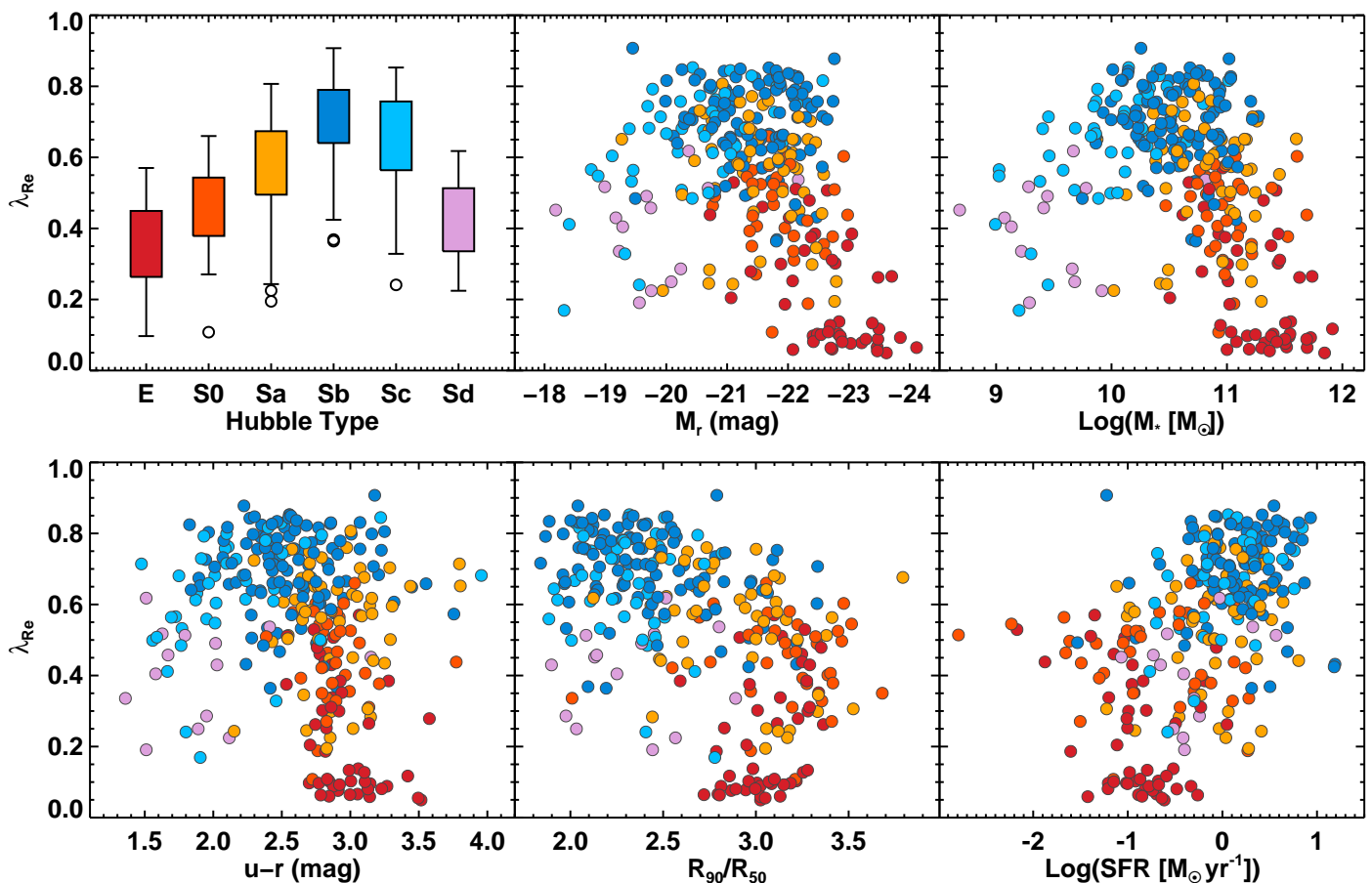
Fig. 5 \lambda_{Re} relations with global parameters for the sample of 300 CALIFA galaxies. Galaxies are color-coded with Hubble type. The top left panel shows a whisker plot enclosing the interquartile range (IQR), defined at IQR25%-IQR75% for galaxies of each morphological type. The whiskers extend out to the maximum or minimum value of the data, or to 1.5 times IQR25% or IQR75% in case there is data beyond this range. Outliers are identified with small circles. Other panels show relations with r -band absolute magnitude M_r , total stellar mass M_* , u - r Petrosian color, concentration index R_{90}/R_{50} , and star formation rate SFR. See text for details.
