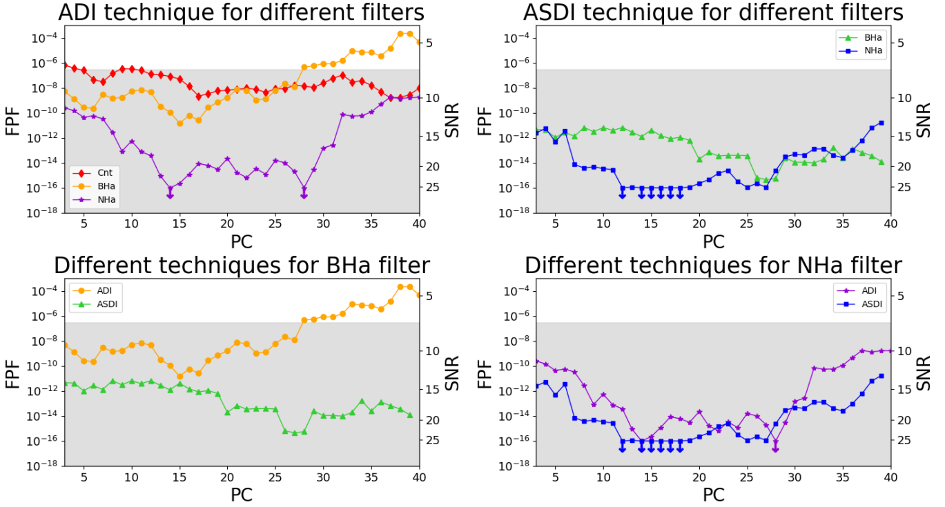
Fig. B.1. Performance comparison for H \alpha imaging with SPHERE/ZIMPOL using different filters (narrow and broad H \alpha ) and reduction techniques (ADI and ASDI) based on the HD142527 dataset. In all panels the FPF obtained for HD142527 B is shown, as a function of the number of subtracted PCs used in PynPoint. On the right side of each panel we give the scale of the S/N to improve understanding of the plot and to compare different instrumental setups. We note again that this does not correspond to the classical \sigma notation. The gray regions indicates a confidence level for the detection of HD142527 B of at least 99.99995%, i.e., >5\sigma in case of Gaussian noise. Because of the applied corrections for small sample statistics, the border of the gray area does not correspond to an S/N of 5.
