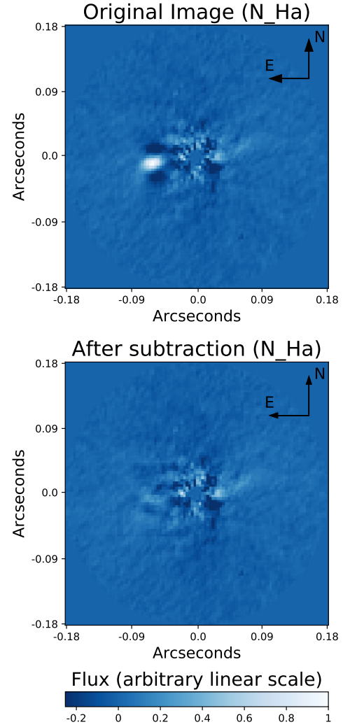
Fig. 3. Image of HD142527 before (top panel) and after (bottom panel) the insertion of the negative companion resulting from the Hessian matrix algorithm. The image flux scale is the same in both images. In this case 14 PCs were subtracted and a mask of 10.8 mas (radius) was applied on the 101 \times 101 pixels images of the N_Ha stack.
