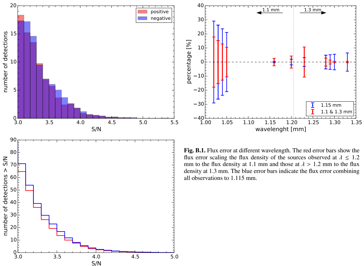
Fig. A.1. Top: number of positive (red) and negative (blue) sources detected in 300 continuum pure noise maps and normalised for 18 continuum maps. Bottom: cumulative distribution of positive (red) and negative (blue) detections.
