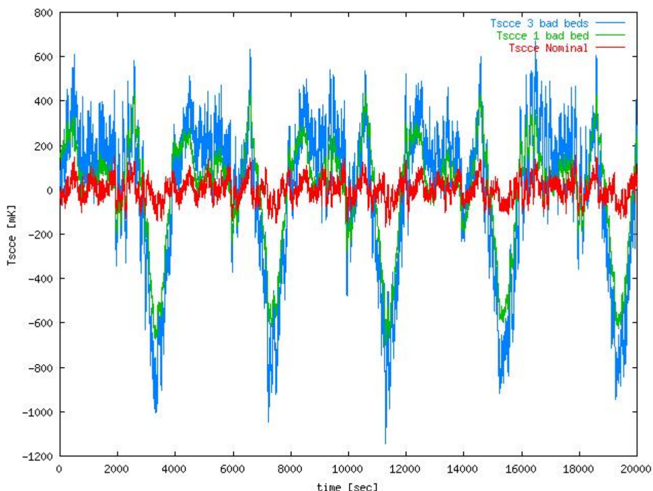
Figure 6 TODs of T_{scee} for the nominal case (red) and simulated for complete degrading of 1 sorption bed (green) and 3 sorption beds (blue).
