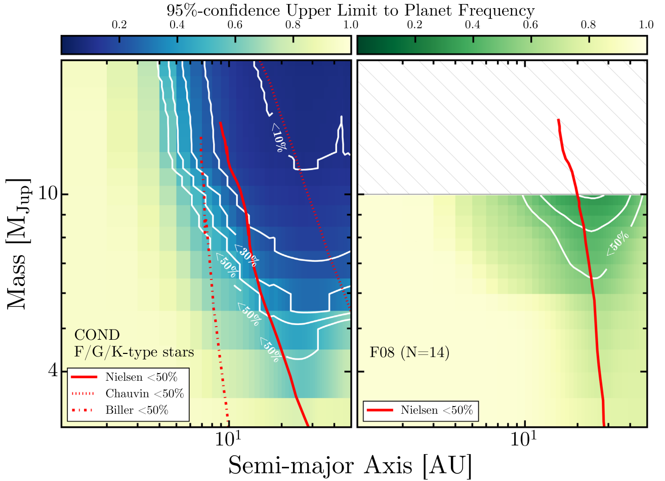
Figure 11. Constraints rederived with classical 5\sigma contrast curves for comparison to earlier surveys. Left: LEECH 95% confidence upper limits to planet frequency around FGK stars as a function of orbital semimajor axis and planet mass using COND evolutionary models and our classical 5\sigma contrast curves, blue color map, and white contours. We overplot, in red, the 50% upper-limit contour from three other surveys that publish similar maps for target lists with similar spectral-type distributions (Nielsen & Close 2010; Biller et al. 2013; Chauvin et al. 2015). LEECH provides the best constraints at small semimajor axes. Right: same as for the left panel but for the F08 models. Here we compare to Nielsen & Close (2010), who reported results for a similar spectral-type distribution mainly consisting of FGK stars. LEECH provides the best constraints on cold-start planets interior to \sim 20 au.
