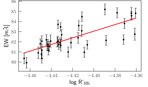
Figure 2. Same of Fig. 1-Top, but here Voigt profiles have been used to measure the EWs of the Ba II line instead of Gaussians.
