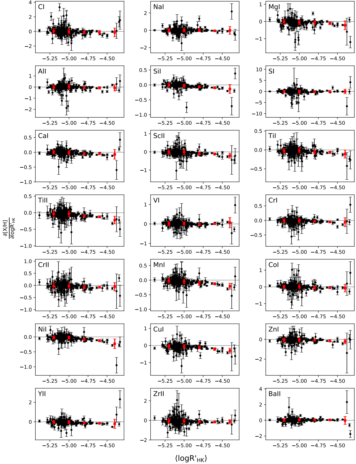
Figure 5. Each panel shows the sensitivity of the X-element abundance to chromospheric activity (i.e., \partial[X/H]/\partial \log R'_{\text{HK}} ) for all stars in our sample as a function of their typical \log R'_{\text{HK}} index (black dots). Red squares and their error bars represent the binned-averaged \partial[X/H]/\partial \log R'_{\text{HK}} values and standard deviations at different intervals in \langle \log R'_{\text{HK}} \rangle .
