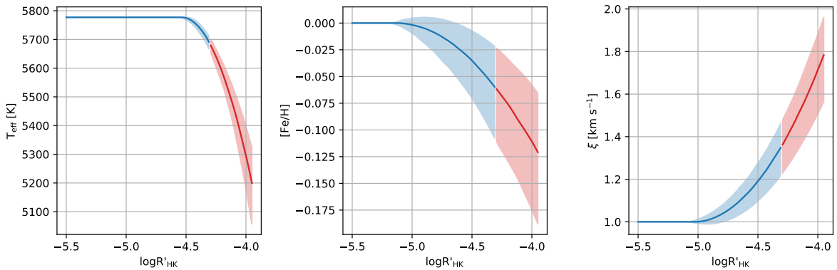
Figure 4. The three panels describe how the stellar parameters T_{\text{eff}} , [\text{Fe}/\text{H}] , and \xi vary as a function of the stellar activity based on the model described in Eq. 2 and the posteriors' distributions obtained through the MCMC simulation. The blue areas represent the 90% confidence intervals within the range of \log R'_{\text{HK}} indexes covered by the stars in our sample, while the red areas are the extrapolations of the same model at higher \log R'_{\text{HK}} values. The solid lines represent the maximum a posteriori estimates. No variation is expected for \log g .
