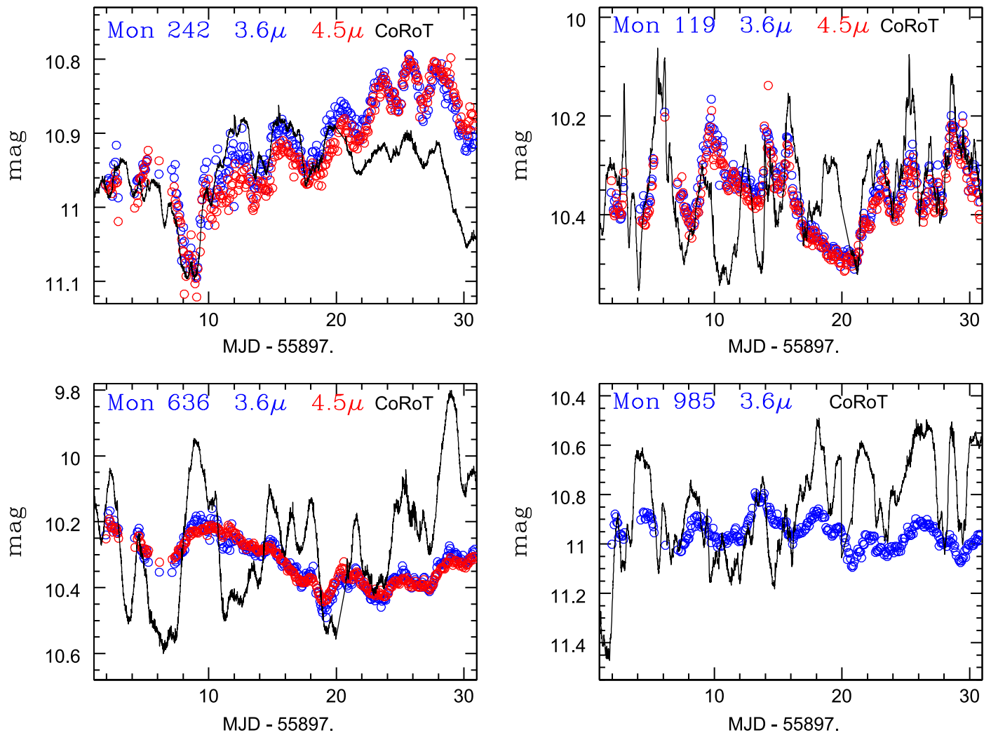
Figure 18. Overlay of the CoRoT and Spitzer light curves for four of the stochastic light curve stars. The plots are arranged according to their disk-to-photosphere flux ratio at 4.5 \mu\text{m} , from least disk-dominated at top-left (Mon-242) to most disk-dominated at bottom-right (Mon-985). This results in their also being approximately ordered according to the degree of similarity between the optical and IR light curve structures. For each panel, the optical data are shifted in zero-point to align vertically with the IR data—the optical and IR delta-mag for full scale is the same.
