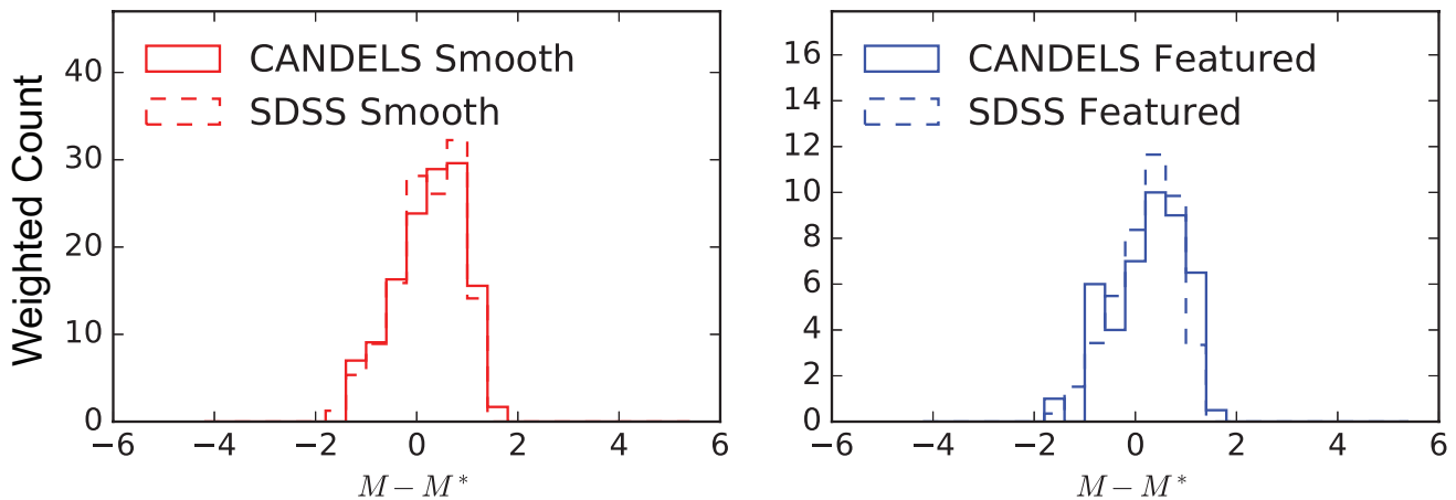
Figure 12. Weighted distributions of M - M^* for the smooth (left panel) and featured (right panel) samples shown in figure 11. M is the galaxy absolute rest-frame magnitude in V (CANDELS) or g (SDSS), and M^* is the “knee” of the luminosity function in the relevant band, evaluated at the redshift of each observed galaxy. The weights for each galaxy in each bin are chosen so that all samples have statistically indistinguishable M - M^* distributions. Weights are normalised separately for smooth and featured distributions and chosen so that the maximum weight for any single galaxy is 1.0; this results in effective counts of 132 galaxies per smooth sample and 44 galaxies per featured sample (CANDELS and SDSS are shown as solid and dashed curves, respectively). The peak of the distribution is slightly fainter than M^* at each redshift, and the full weighted distribution includes galaxies at luminosities \pm 2 magnitudes from M^* . The bulge properties of these weighted samples are compared in Figure 13.
