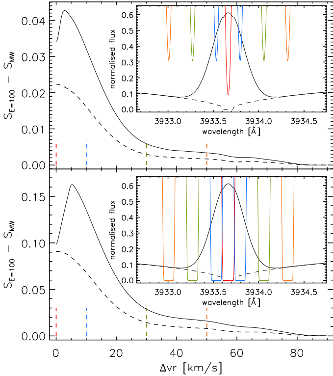
Fig. 11. Top: difference between the reference S value S_{E=100} calculated without ISM absorption, and S_{\text{MW}} obtained considering two non-saturated ( \log N_{\text{CaII}} = 11.5 ) ISM absorption components as a function of velocity separation ( \Delta v in \text{km s}^{-1} ) of each ISM feature from the line centre. With increasing \Delta v , the two features move in opposite directions. The black dashed line shows the case of a single ISM absorption component moving redwards of the line centre. The short dashed vertical lines are colour-coded by the absorption features shown in the insert and indicate their position relative to the line centre. The insert shows the photospheric plus chromospheric flux (the photospheric spectrum is shown by a dashed line) in black and, as an example, absorption components lying at a velocity separation of 0.0 (red), \pm 10.0 (blue), \pm 30.0 (green), and \pm 50.0 (orange) \text{km s}^{-1} from the line centre. Bottom: as the top panel, but considering saturated ( \log N_{\text{CaII}} = 14.0 ) ISM absorption lines.
