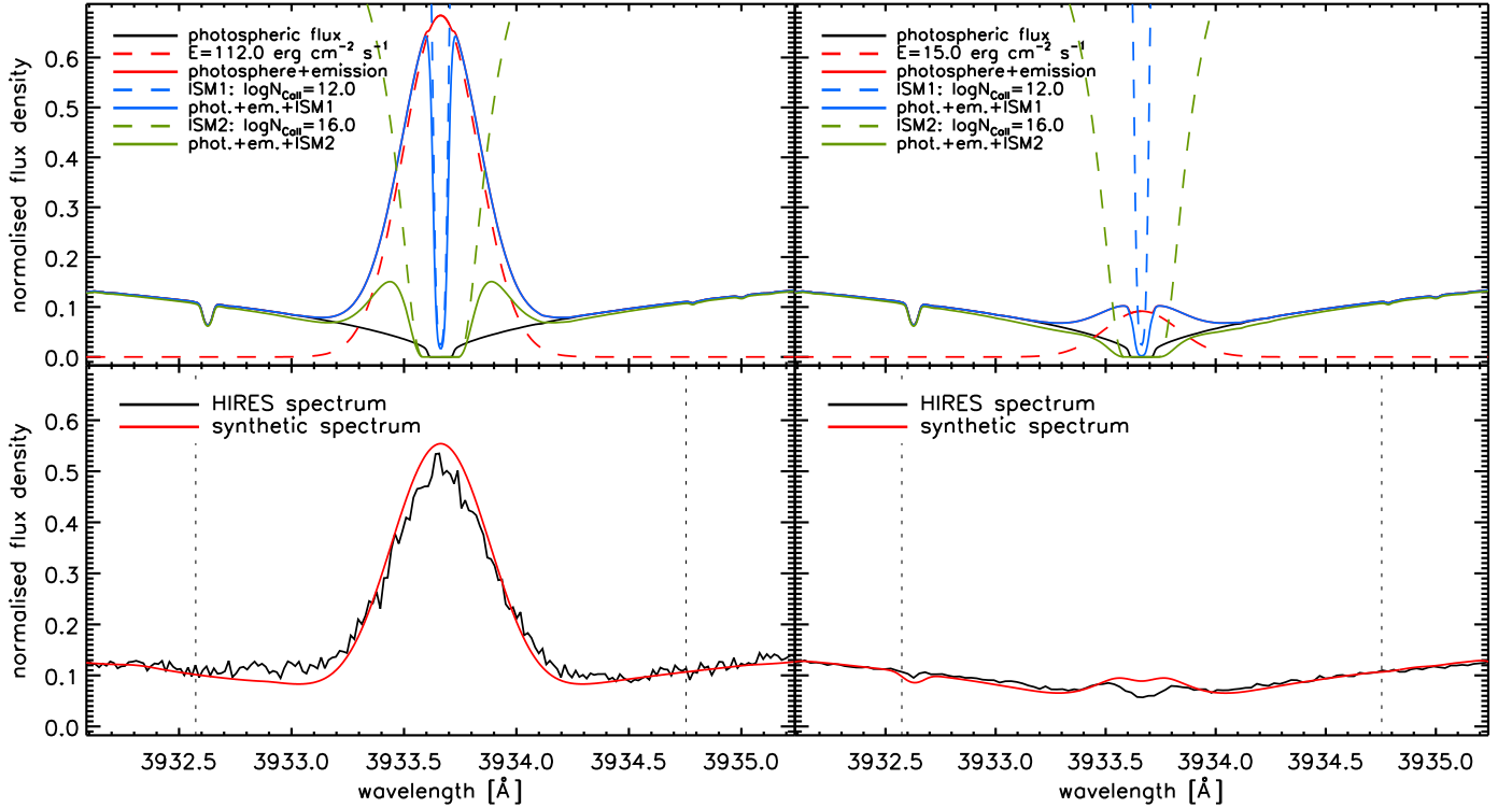
Fig. 2. Top left: LLmodels photospheric spectrum of the Sun in the region of the Ca II K line core (black solid line) modified by adding a line core emission of 112 \text{ erg cm}^{-2} \text{ s}^{-1} (red solid and dashed lines). This composite spectrum has then been modified by two ISM absorption features, located at the line centre, calculated with Ca II column densities of 10^{12} and 10^{16} \text{ cm}^{-2} (blue and green dashed and solid lines). Bottom left: comparison of a high resolution Hires spectrum of the young Sun-like star EK Dra and the corresponding synthetic spectrum obtained by adding a line core emission of E = 112 \text{ erg cm}^{-2} \text{ s}^{-1} to the photospheric spectrum. The two spectra return the same S_{\text{MW}} value of 0.440. The synthetic spectrum accounts also for the instrumental spectral resolution and the stellar projected rotational velocity ( \approx 15 \text{ km s}^{-1} ). Right: same as the left panels, but for the hyper-velocity halo Sun-like star HD 29587. In this case, the emission flux is 15 \text{ erg cm}^{-2} \text{ s}^{-1} , corresponding to a S_{\text{MW}} value of 0.144. The synthetic spectrum does not match the line profile in detail, possibly due to non-LTE effects, but it reproduces the empirical S value. In the top panels, the red solid lines are visible just in the very core of the line, as it is otherwise covered by the blue solid line.
