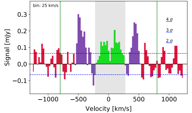
Fig. 4. Similar to the central panel of Fig. 3b, the 25 \text{ km s}^{-1} -binned stacked [C II] residuals of the high-SFR group are shown. However, here, for the five rotators in the subsample, R_{i,k} (see Eq. (1)) is calculated by subtracting a kinematic model to the observed spectra. We color in green the channels where the residuals left by the tilted-ring fit are non-null, specifically in the velocity range v \sim [-225; +275] \text{ km s}^{-1} , marked by the gray shaded region.
