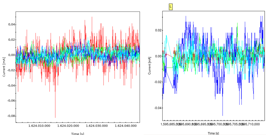
Figure 5 – Feed 22 FEM Id S2 (red), Id S1 (green), Id M1 (blue), and Id M2 (cyan). Left panel: CPV stability check. Right panel CSL test XXX_0203. On the right panel the S2 drain current is shown in blue
