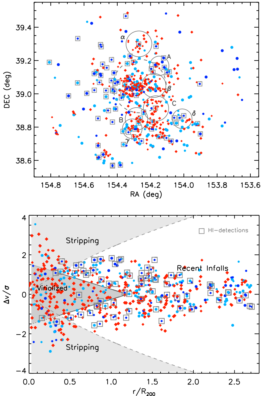
Figure 8. Spatial (top) and phase-space (bottom) distribution of all the cluster galaxies, colour-coded by NUV - R and sized by luminosity as in Fig. 2. The open grey squares correspond to the H I -detected galaxies. Open circles in the top panel mark the groups defined in Fig. 4 and the dashed circle the R_{200} of A963_1. Shaded areas in the bottom panel indicate several regions of interest such as the ‘recent infall’, ram-pressure ‘stripping’, and ‘virialized’ regions, discussed in the text. A colour version of this figure is available in the online version of the paper.
