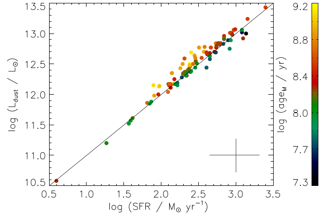
Figure 9. Median-likelihood estimates of the star formation rate against the total dust infrared luminosity of the ALESS sources. The black line shows the relation of Kennicutt (1998; scaled to a Chabrier 2003 IMF) which essentially assumes an optically thick starburst.
