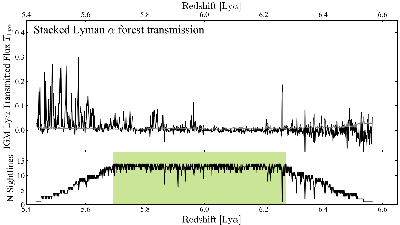
Figure 2. Top—The stacked Ly \alpha forest spectrum (black) of 14 ASPIRE quasar sightlines used in our analysis, adopting a redshift grid of dz = 0.001 from z = 5.435 to z = 6.568 . The spectral uncertainty of the stacked spectrum is shown in gray. Bottom—The number of quasar lines of sight (LOSs) available in each pixel of the redshift grid. Nearly all quasars used in this work cover the z \sim 5.70 – 6.27 Ly \alpha forest (the green-shaded region). Some pixels are strongly influenced by sky OH emission lines, therefore, they have been removed in the analysis, resulting in troughs shown in the number of quasar LOSs.
