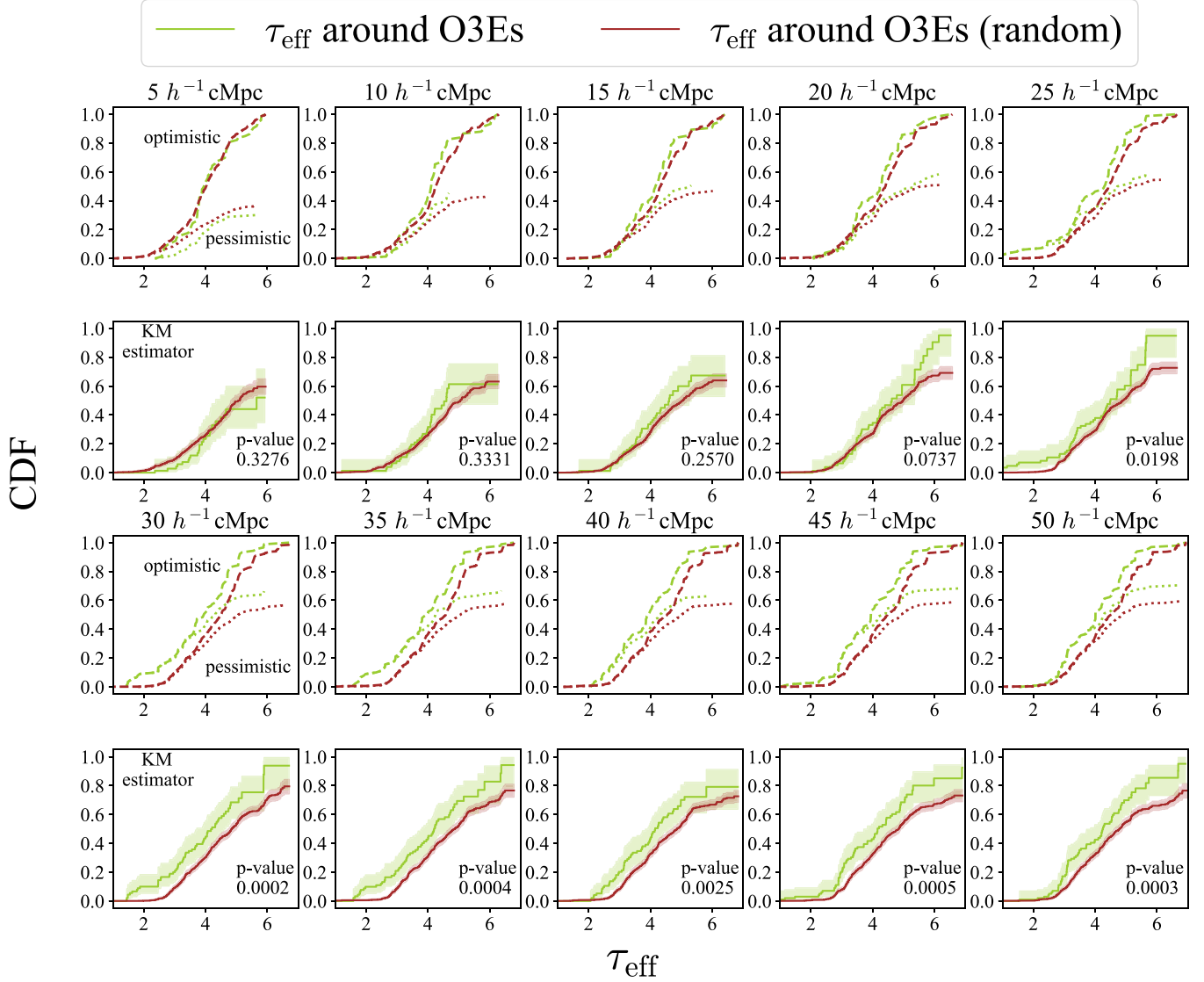
Figure 9. The first and the third rows show the CDFs of the \tau_{\text{eff}} around [O III] emitters at 5.4 < z < 6.1 (yellow-green), adopting influence radii from 5 h^{-1} cMpc to 50 h^{-1} cMpc. The random cumulative distribution function of the \tau_{\text{eff}} around [O III] emitters is shown in brown, representing the \tau_{\text{eff}} distribution of IGM patches. The optimistic and the pessimistic CDFs are plotted in dashed and dotted lines, respectively. The second and the fourth rows show the fitted CDFs from the KM estimator and the 1\sigma confidence interval of the CDF is shown in the shaded regions of the corresponding color. The null hypothesis p -value from the log-rank test is shown in the bottom right corner of each subpanel. See the text for more details.
