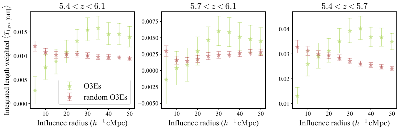
Figure 12. Average transmitted flux around [O III] emitters (filled yellow-green stars), weighted by the integrated length of each \tau_{\text{eff},[\text{O III}]} measurement, as a function of influence radii at 5.4 < z < 6.1 , 5.7 < z < 6.1 , and 5.4 < z < 5.7 . The 1\sigma uncertainty is calculated using bootstrapping. The random values are denoted by filled brown stars.
