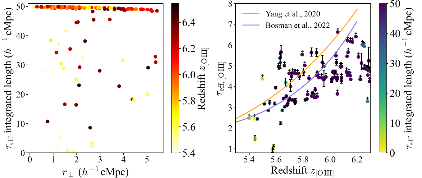
Figure 5. Left—The integrated path length for \tau_{\text{eff, [O III]}} measurements as a function of the transverse distance ( r_{\perp} ), adopting an influence radius of 25 h^{-1} cMpc. Each point is color-coded by the redshift of the [O III] emitter z_{[\text{O III}]} . Except for those [O III] emitters at the boundary of the Ly \alpha forest, for most [O III] emitters, the integrated length for \tau_{\text{eff, [O III]}} measurements is \sim 50 h^{-1} cMpc. Right—The \tau_{\text{eff}} around the [O III] emitters ( \tau_{\text{eff, [O III]}} ) adopting an influence radius of 25 h^{-1} cMpc, as a function of the [O III] emitter redshift z_{[\text{O III}]} . The integrated path length for each \tau_{\text{eff, [O III]}} measurement is color-coded. The best-fit \tau_{\text{eff}} redshift evolution from J. Yang et al. (2020b) and S. E. I. Bosman et al. (2022) is denoted by the orange and purple lines, respectively.
