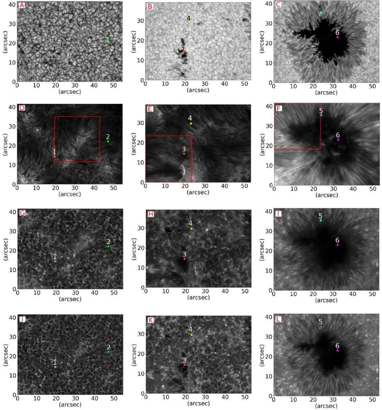
Figure 2. CRISP Fe I 6302 Å continuum images (panels A–C) and CHROMIS Ca II K 3933 Å images in the line core (panels D–F), at -0.42 Å from the line core at roughly K_{1V} (panels G–I), and at +1.05 Å in the red wing (panels J–L) of the three regions analysed in our study, referring to a quiet Sun area (left column panels), an active region with plages and several pores (middle column panels), and a sunspot with umbra and penumbra (right column panels). After the image processing described in Sect. 2.2, the CRISP and CHROMIS observations are shown here with same dimension and pixel scale, which in the original data are in favour of the CHROMIS observations and is maintained here. Each observation is shown using the intensity interval that enhances the visibility of the solar features therein. The small coloured boxes show the six 20 \times 20 pixels wide areas randomly selected in the observations to represent the solar features analysed in our study in the ambient to which they belong. The boxes are shown in all panels to make comparisons easier. The red boxes on line core observations mark the regions shown in Figs. 5, 7, and in Appendix B.
