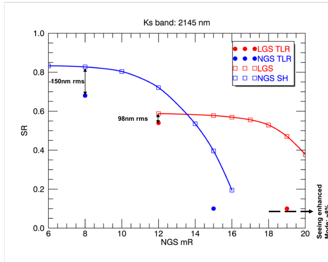
Figure 6 Estimated performance in Ks-band of the ERIS AO system
