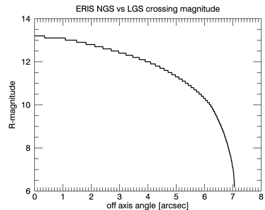
Figure 8 Transition magnitude vs NGS off-axis angle. Below the curve NGS-mode performs better than LGS-mode; the opposite above the curve.
