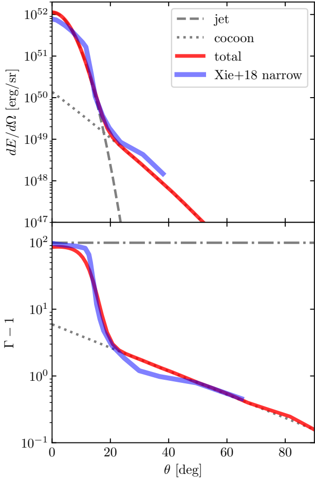
Fig. A.3. Same as Fig. A.2, but for the “narrow engine” case in Xie et al. (2018) (we choose the structure extracted from the 10^4 s snapshot as shown in their Fig. 2, right-hand panels).
