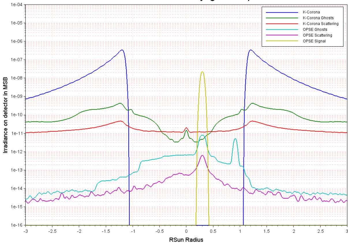
Figure 26. Comparison with In-FoV Straylight
