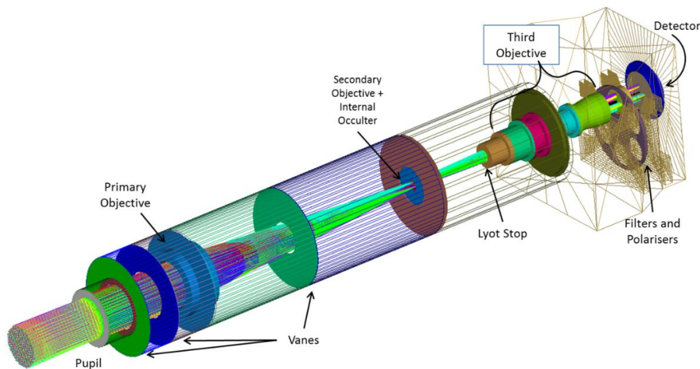
Figure 3 - Mechanical Model
