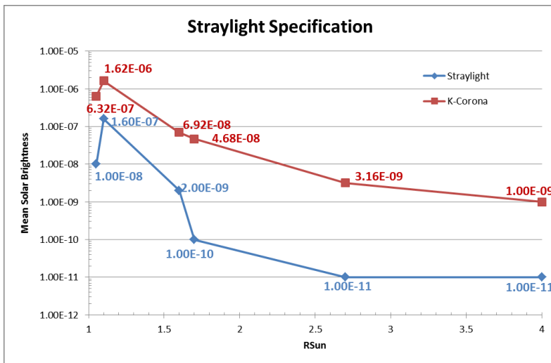
Figure 8 - Straylight Specification
