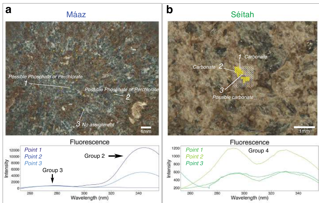
Extended Data Fig. 6 | Group 3 Feature Mineral Association in Bellegarde and Group 4 Feature -290 & 330 nm Feature and Mineral Associations in Garde. A) Colorized ACI of Bellegarde (Máaz fm.) HDR scan on sol 186 with laser overlay (gray = no fluorescence detected, yellow = fluorescence at -270–295 nm detected). Three points of interest with Group 3 fluorescence are marked in white and correlate to the smoothed mean spectra below. Point 1 and 2 were co-located with a potential phosphate or perchlorate detection ( -973 , -965 \text{cm}^{-1} );
