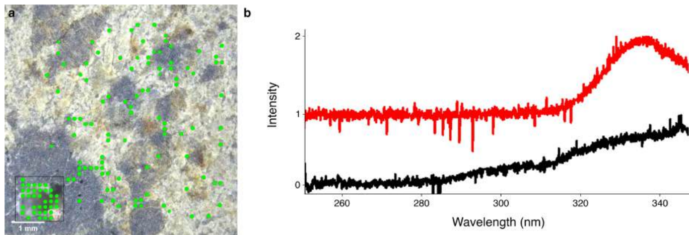
Extended Data Fig. 5 | Mean Fluorescence Spectra on Two Regions of Meteorite Calibration Target. A) Colorized ACL image from a survey scan of the meteorite calibration target from sol 181. Green spots represent the relative laser beam diameter that have a positive identification for the ~335–350 nm
