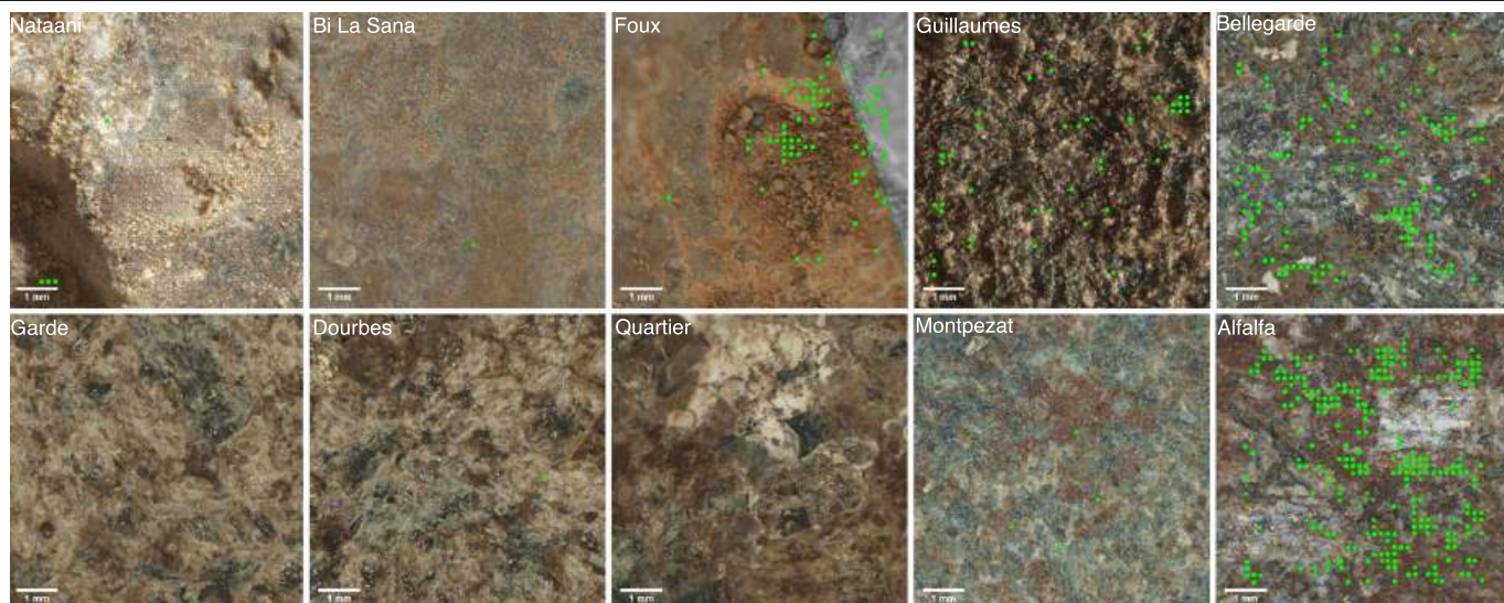
Extended Data Fig. 2 | Group 3 Fluorescence Across All Targets Analyzed by SHERLOC. Colorized ACL images from survey scans of each of the 3 natural targets (top left), 4 Máaz abraded targets (right), and 3 Séítah abraded targets
