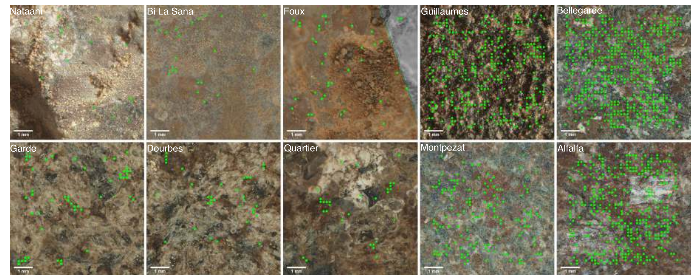
Extended Data Fig. 1 | Group 2 Fluorescence Across All Targets Analyzed by SHERLOC. Colorized ACL images from survey scans of each of the 3 natural targets (top left), 4 Máaz abraded targets (right), and 3 Séítah abraded targets
