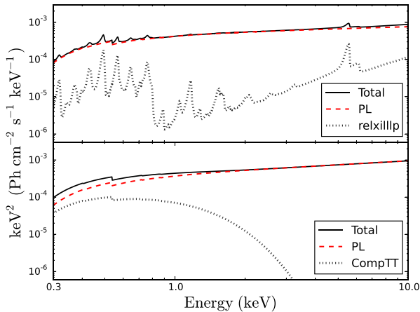
Figure 3. Best-fitting models to the XMM-Newton spectra for the cases where reflection (top panel) and Comptonization (bottom panel) contribute to the spectra. The solid, black line is the total model, the red, dashed line is the power-law emission from the jet, while the dotted, grey line shows the contribution from reflection or Comptonization. Both models also include Galactic absorption.
