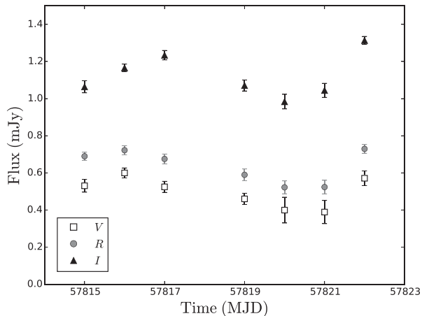
Figure 6. Optical light curve of FBQS J1644+2619 from the monitoring with REM during 2017 March 3–10. Open squares, grey circles, and black triangles show the extinction-corrected fluxes in the V, R, and I bands, respectively.
