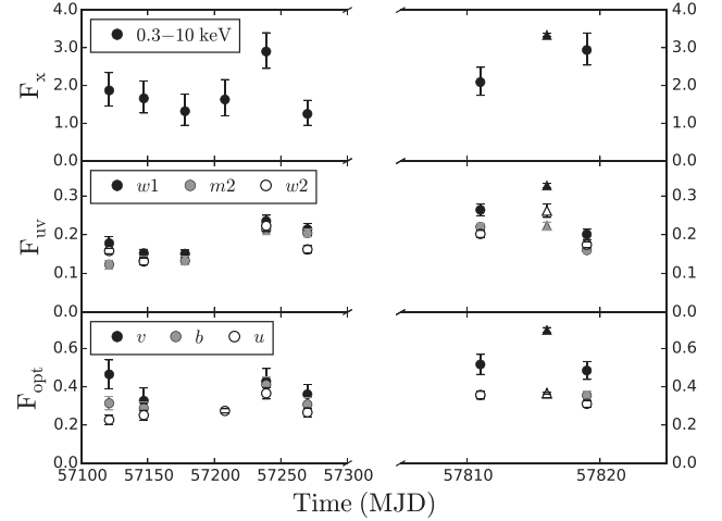
Figure 5. Flux evolution of FBQS J1644+2619 during 2015 April 9–September 5 (first part of x -axis) and 2017 February 27–March 7 (second part of x -axis). Top panel: unabsorbed 0.3–10 keV flux in units of 10^{-12} erg cm -2 s -1 , middle panel: extinction corrected UV fluxes in units of mJy (black: w1 band, grey: m2 band, and white: w2 band), bottom panel: extinction corrected optical fluxes in units of mJy (black: v band, grey: b band, and white: u band). The Swift XRT and UVOT observations are shown as circles, while the XMM-Newton EPIC and OM observations are shown as triangles. Note that some of the error bars are smaller than the plot symbols.
