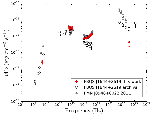
Figure 7. SED of FBQS J1644+2619. Fluxes measured during the XMM-Newton observation are shown in red. These include observations from Medicina, REM, XMM-Newton OM, and EPIC pn, as well as an upper limit from Fermi -LAT. Open symbols are previous observations collected from a variety of observatories and epochs (see the text for details). For comparison, the SED of PMN J0948+0022 is also plotted (grey symbols, from D’Ammando et al. 2015a). The red and grey symbols have error bars that are too small to be seen in the optical–X-ray range. Uncertainties are not plotted for the archival data in the radio–NIR range.
