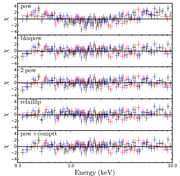
Figure 2. Residuals between the data and the power law, broken power law, double power law, RELXILLLP, and power law+COMP TT models. The best-fitting parameters are provided in Table 3. Data points from pn, MOS1, and MOS2 are shown in black, red, and blue, respectively.
