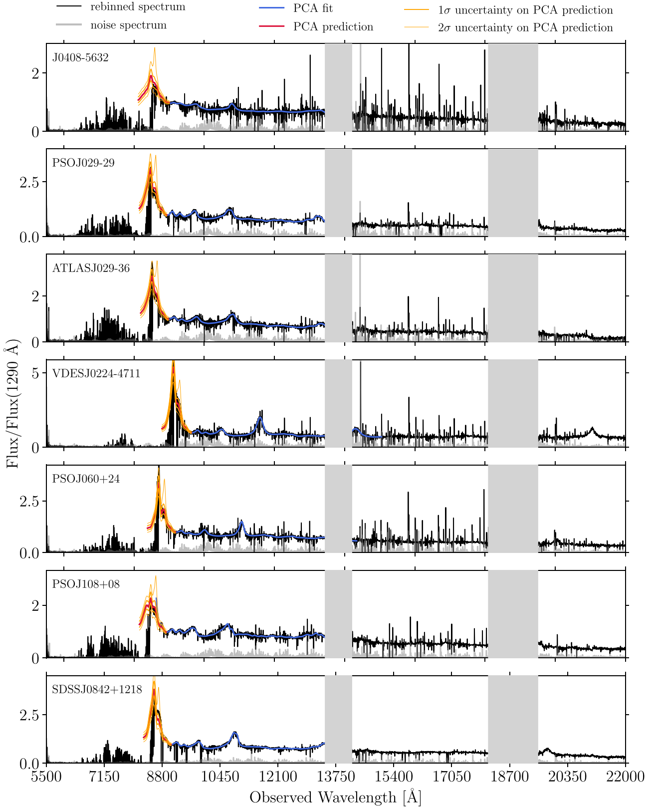
Figure A1. All spectra studied in this paper. Rescaled flux is obtained by dividing with the flux at 1290 \text{\AA} . This rescaled flux, rebinned to 50 \text{ km s}^{-1} , is shown in black. Uncertainty on the flux is shown in grey. Telluric absorption bands are shown in light grey. Best fitting continuum to the redside flux is shown in blue. Predicted blue-side continuum is shown in red. 1\sigma and 2\sigma errors on the continuum predictions are shown in orange.
