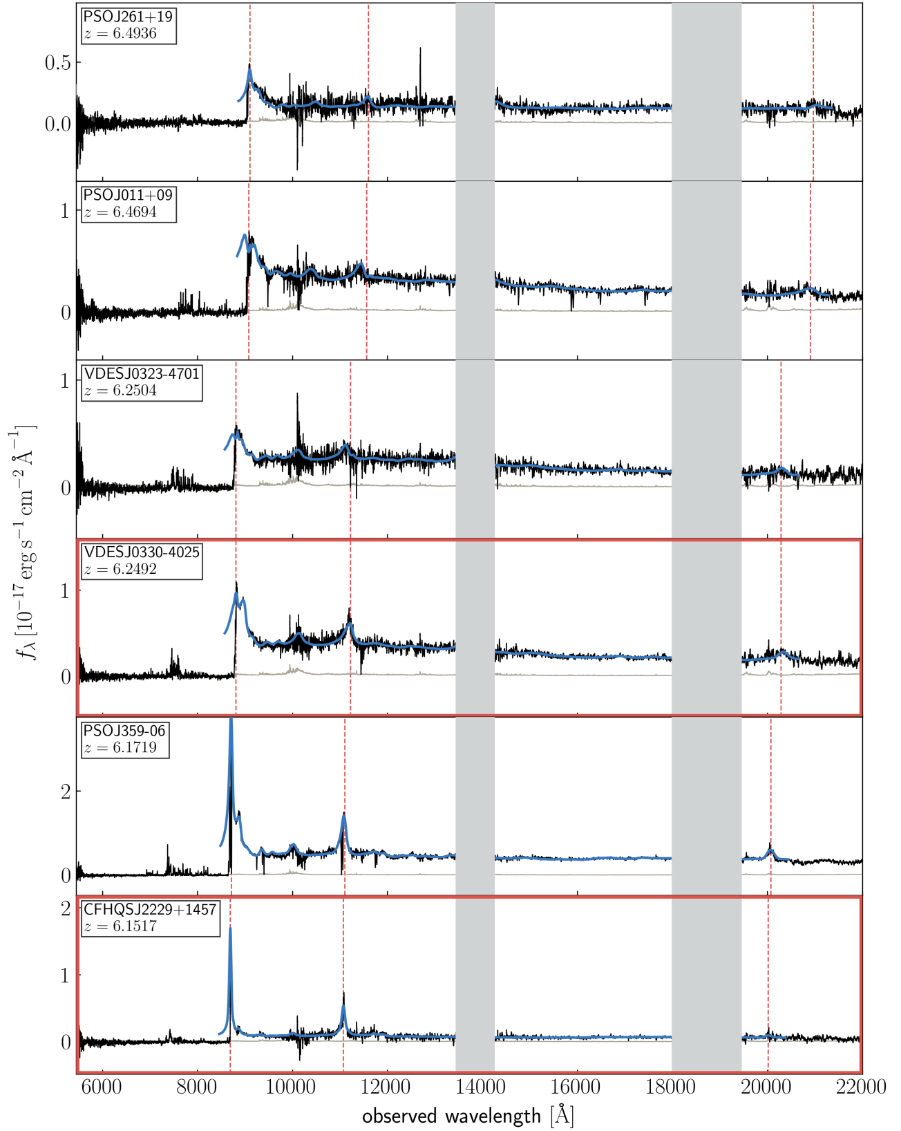
Figure 11. Same as Fig. 2 with quasar continuum estimates, shown in blue.
