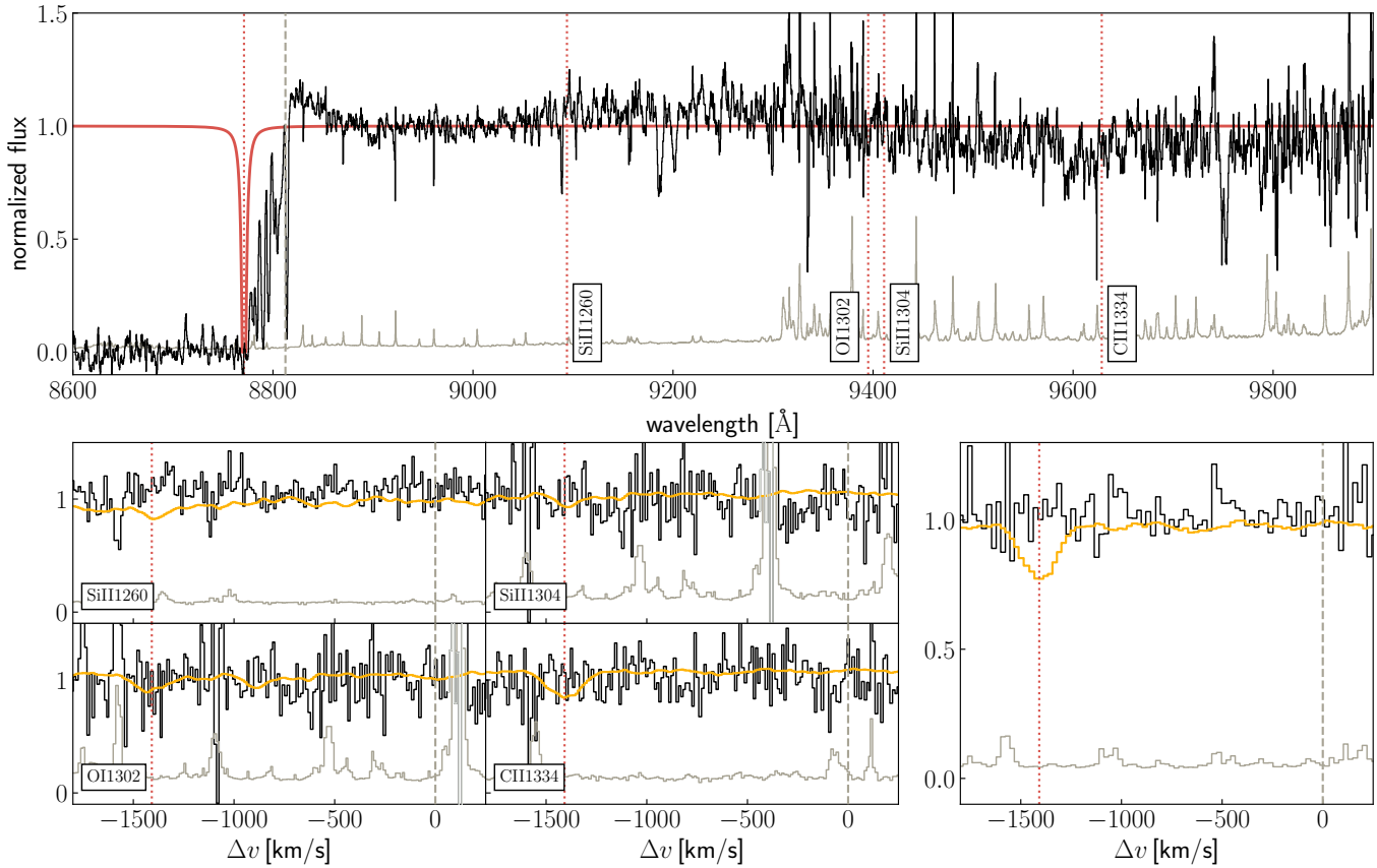
Figure 15. Same as Fig. 6 but for VDES J0330–4025. Wavelength regions around very prominent skylines (shown in light grey) have been masked to avoid biases in the stack.
