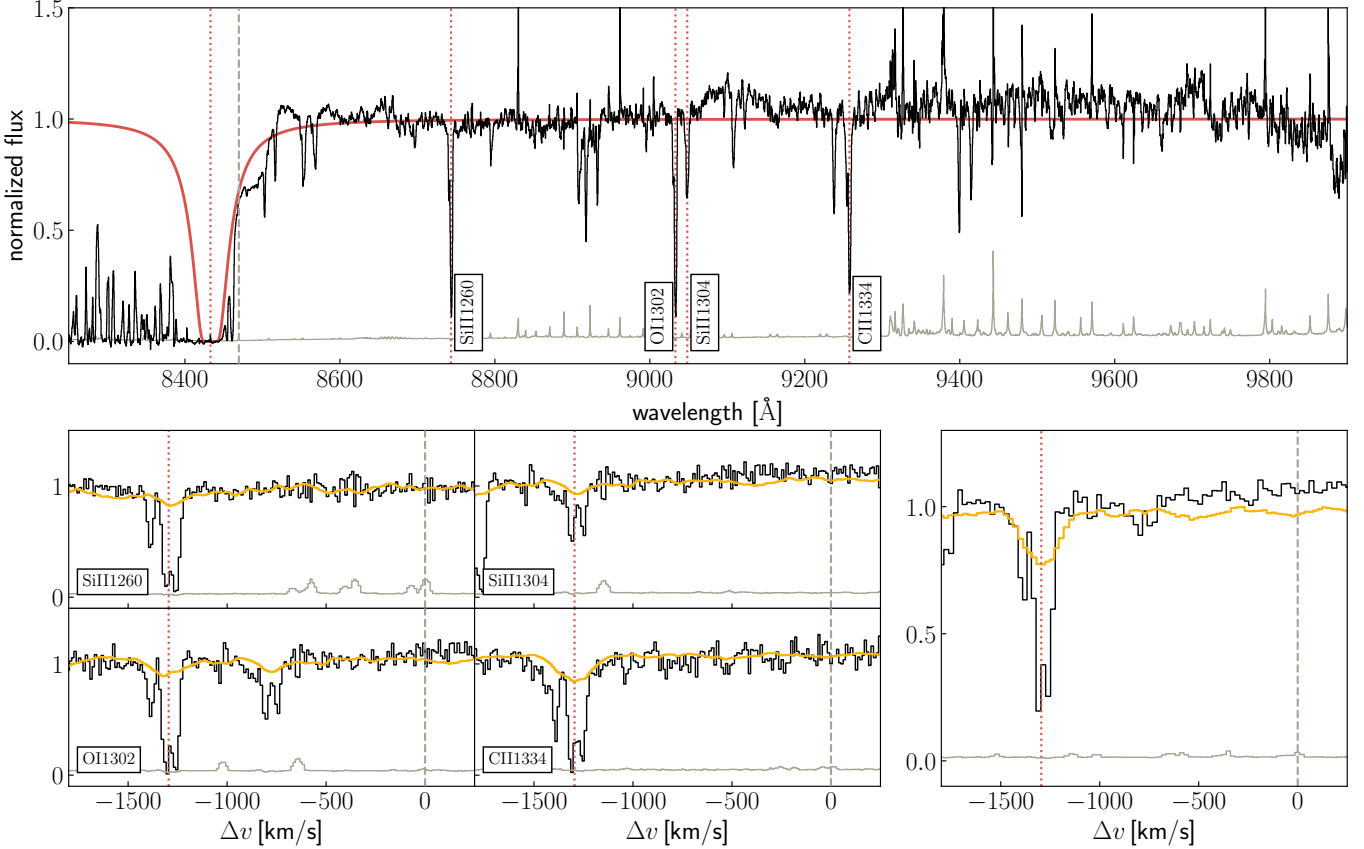
Figure 5. Optical quasar spectrum (black) showing a proximate absorption systems (red) in the vicinity of PSO J056–16 ( top ). The parameters of the absorption system, i.e. \log N_{\text{HI}} = 20.4 \text{ cm}^{-2} and b = 25 \text{ km s}^{-1} , are only fitted by eye. The spectrum at the locations of the low-ionization metal lines ( bottom left ) and the stack thereof ( bottom right ) show clear evidence for the presence an optically thick, self-shielding system. The yellow line represent a composite spectrum of 20 LLSs (Fumagalli et al. 2011).
