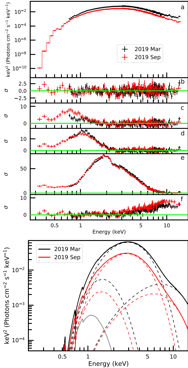
Figure 4. Top panel: the broad-band E^2f(E) unfolded spectra of XTE J1810 from the simultaneous XMM-Newton and NuSTAR observations performed in 2019 March (black) and September (red). The best-fitting 4BB models are plotted with a solid line (see Section 3.2 for more details). Post-fit residuals in units of standard deviations are shown in panel (b). Panel (c): post-fit residuals after setting the normalization of the BB component accounting for the whole NS to zero. Panel (d): post-fit residuals after setting the normalization of the cold BB component to zero. Panel (e): post-fit residuals after setting the normalization of the warm BB component to zero. Panel (e): post-fit residuals after setting the normalization of the hot BB component to zero. Bottom panel: the E^2f(E) plot of the fitted models, with the contributions of the single components. In grey, we plot the BB component that accounts for the emission from the whole stellar surface.
